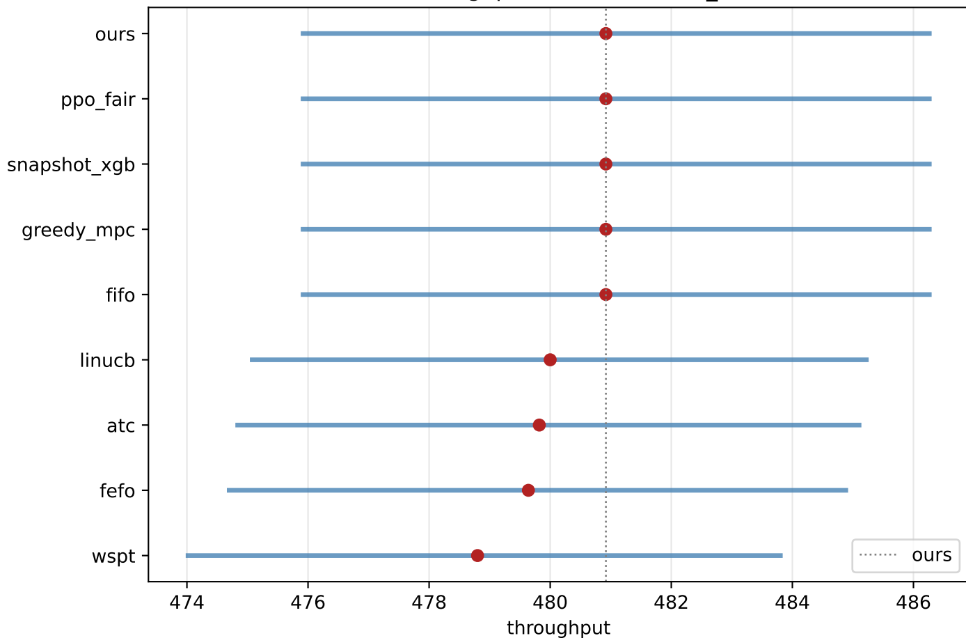
E2 — throughput (scenario=low_load)
