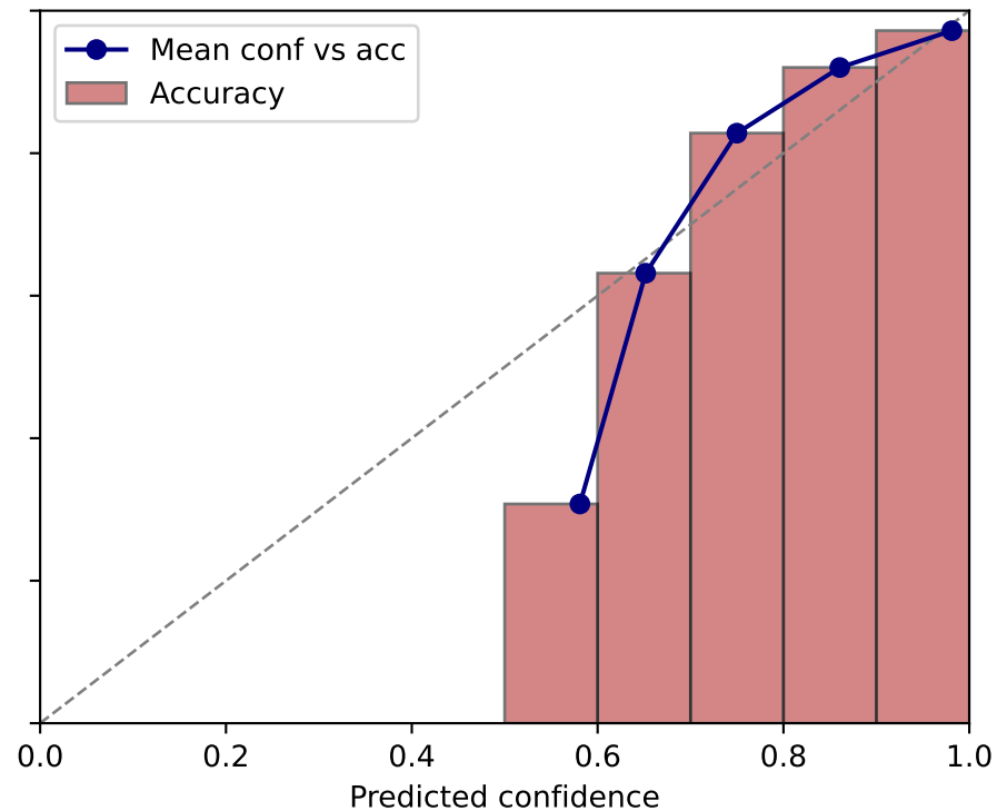
Post-calibration (isotonic) ECE = 0.0281
