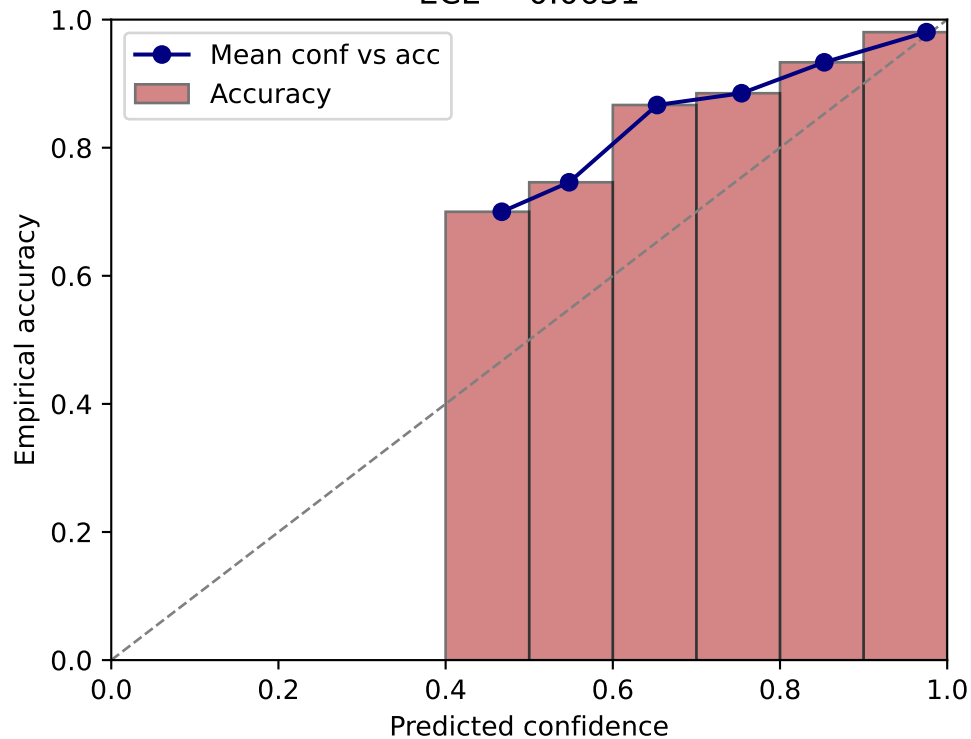
Pre-calibration ECE = 0.0631
