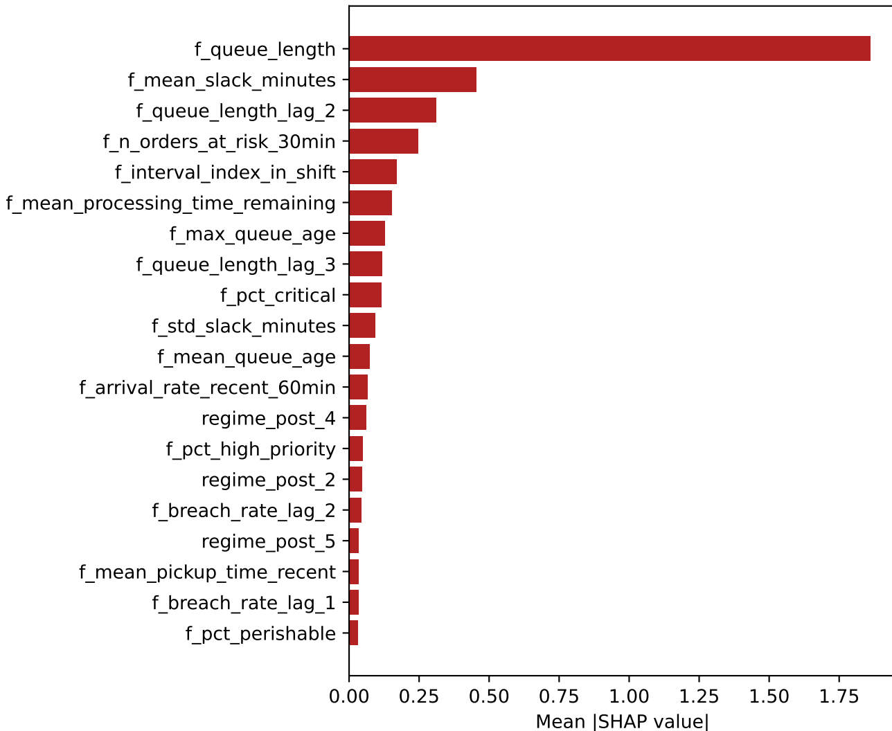
E5 — Global feature importance (top 20)
