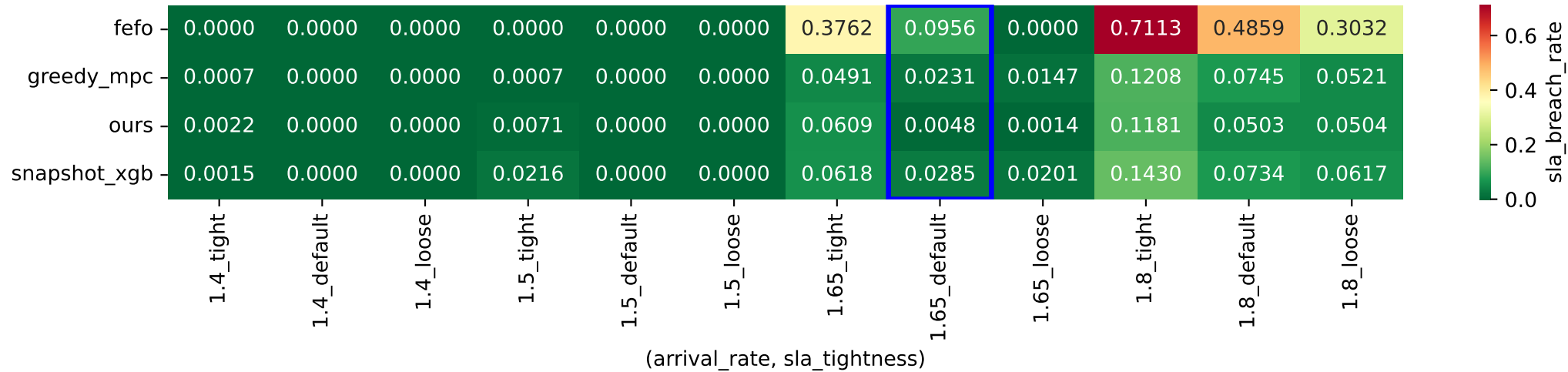
E8 — Robustness Grid: sla_breach_rate
