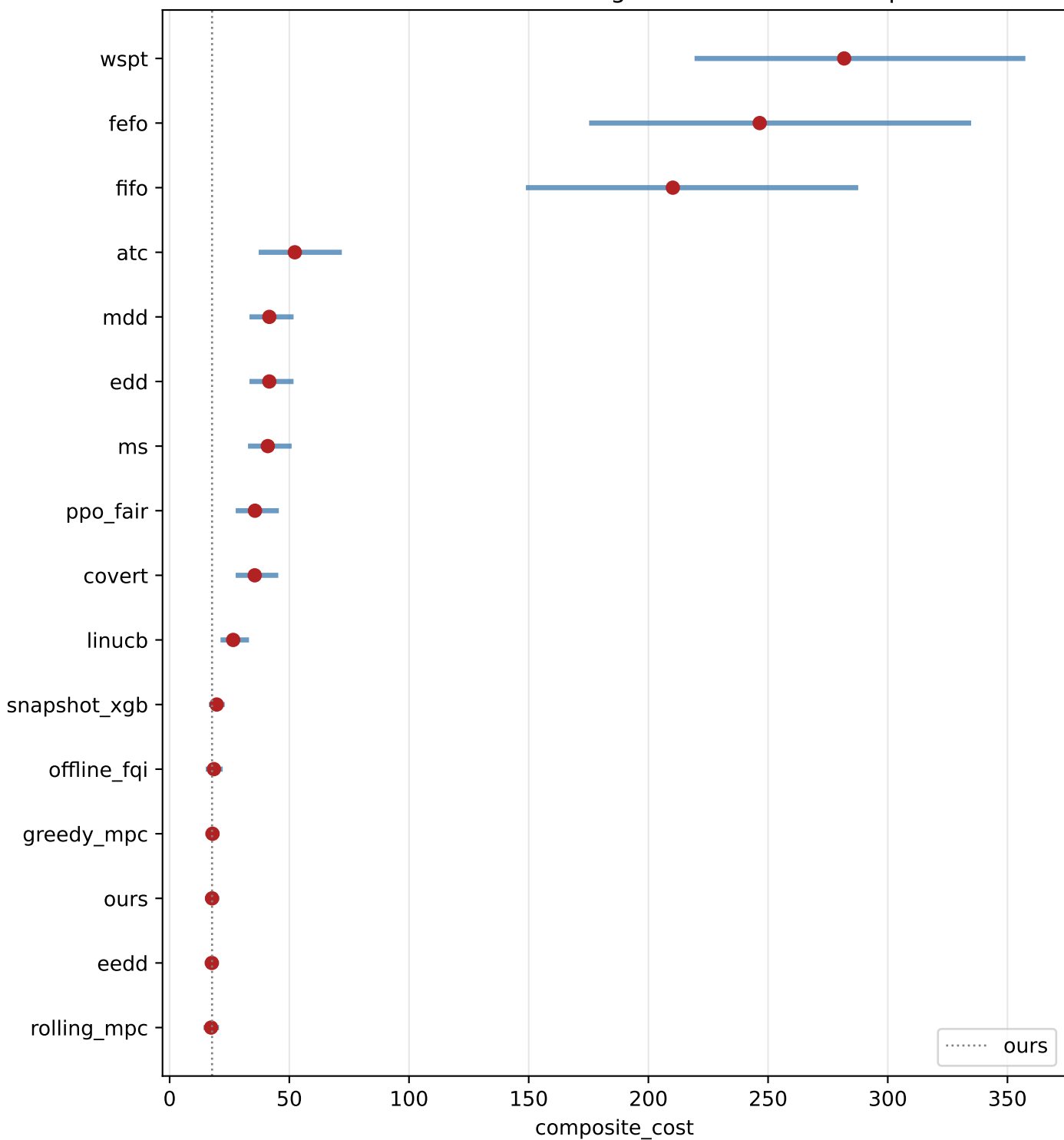
E2 — composite_cost (scenario=balanced) 50 test shifts · 250 training shifts · 95% bootstrap CI
