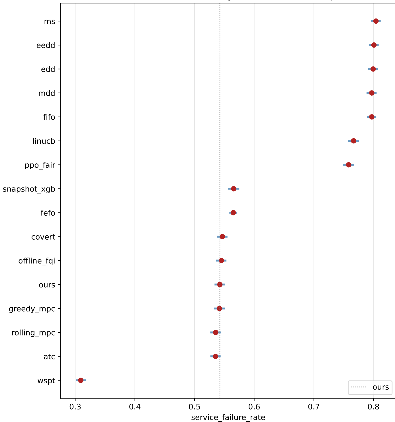
E2 — service_failure_rate (scenario=high_load_perish) 50 test shifts · 250 training shifts · 95% bootstrap CI
