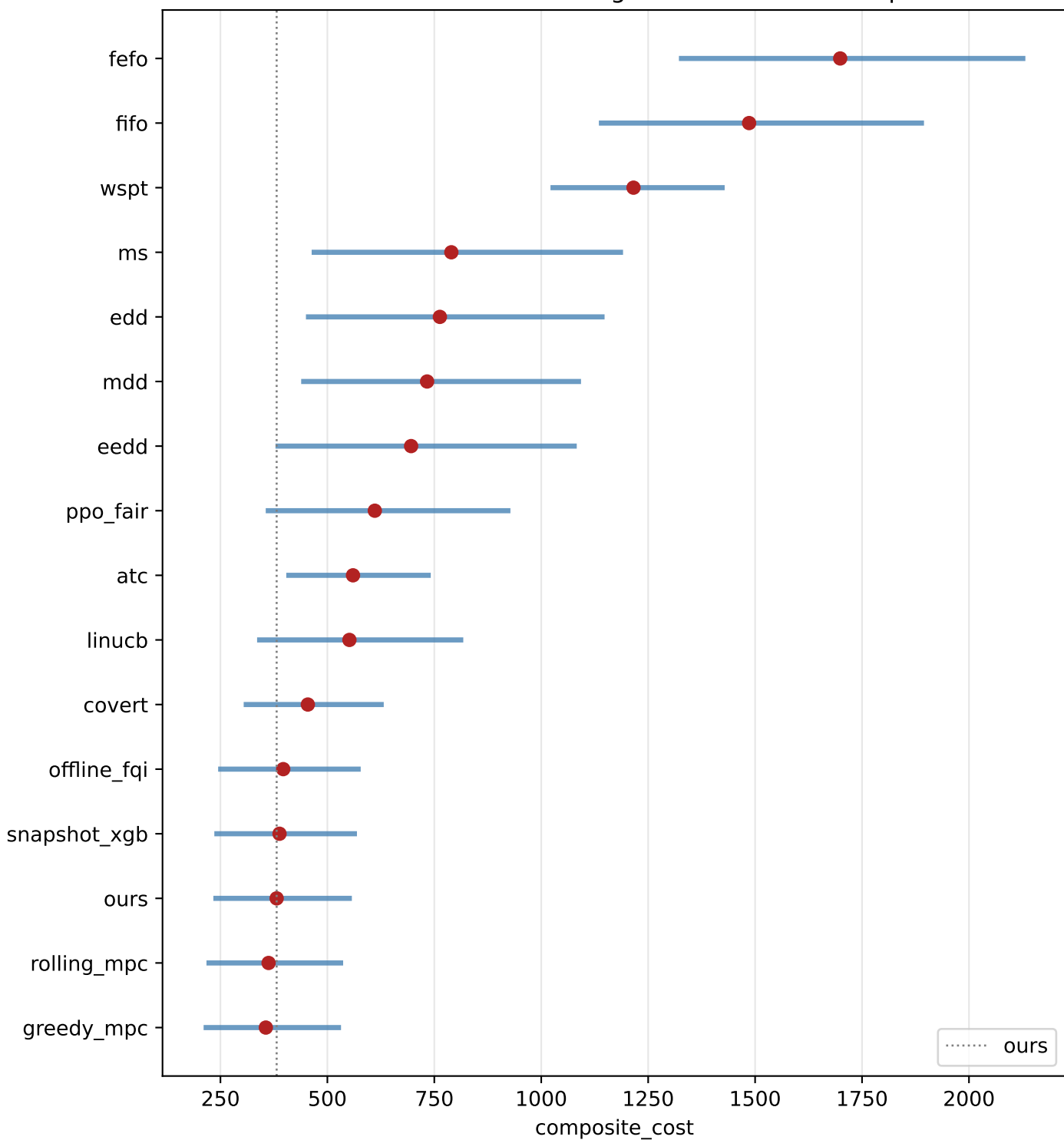
E2 — composite_cost (scenario=default) 50 test shifts · 250 training shifts · 95% bootstrap CI
