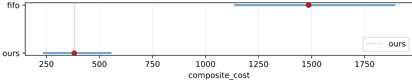
E2 — composite_cost (scenario=default) 50 test shifts · 250 training shifts · 95% bootstrap CI
