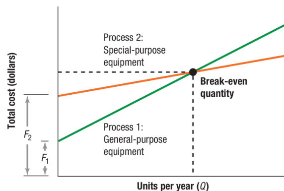
Figure 36: Relationship between process costs and product volume
