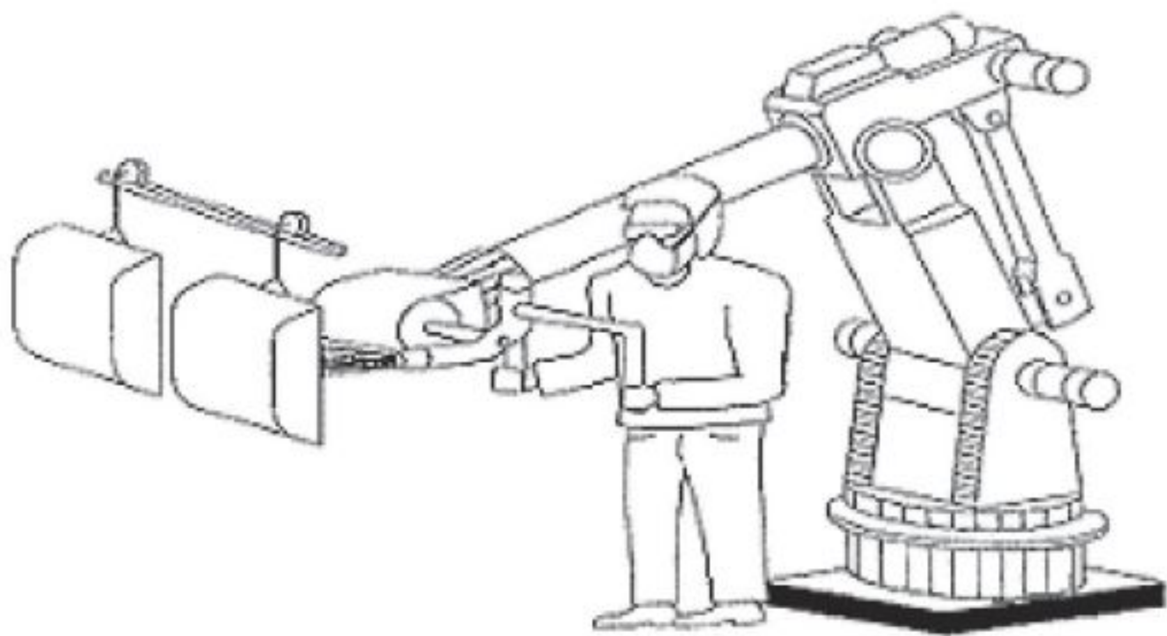
FIGURE 16.3 Walk-through Programming Method.
