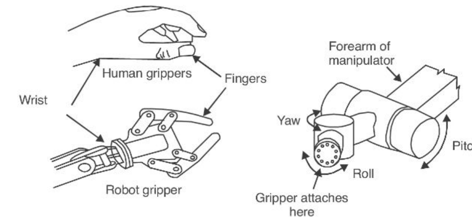
FIGURE 15.3 Robot Gripper.
