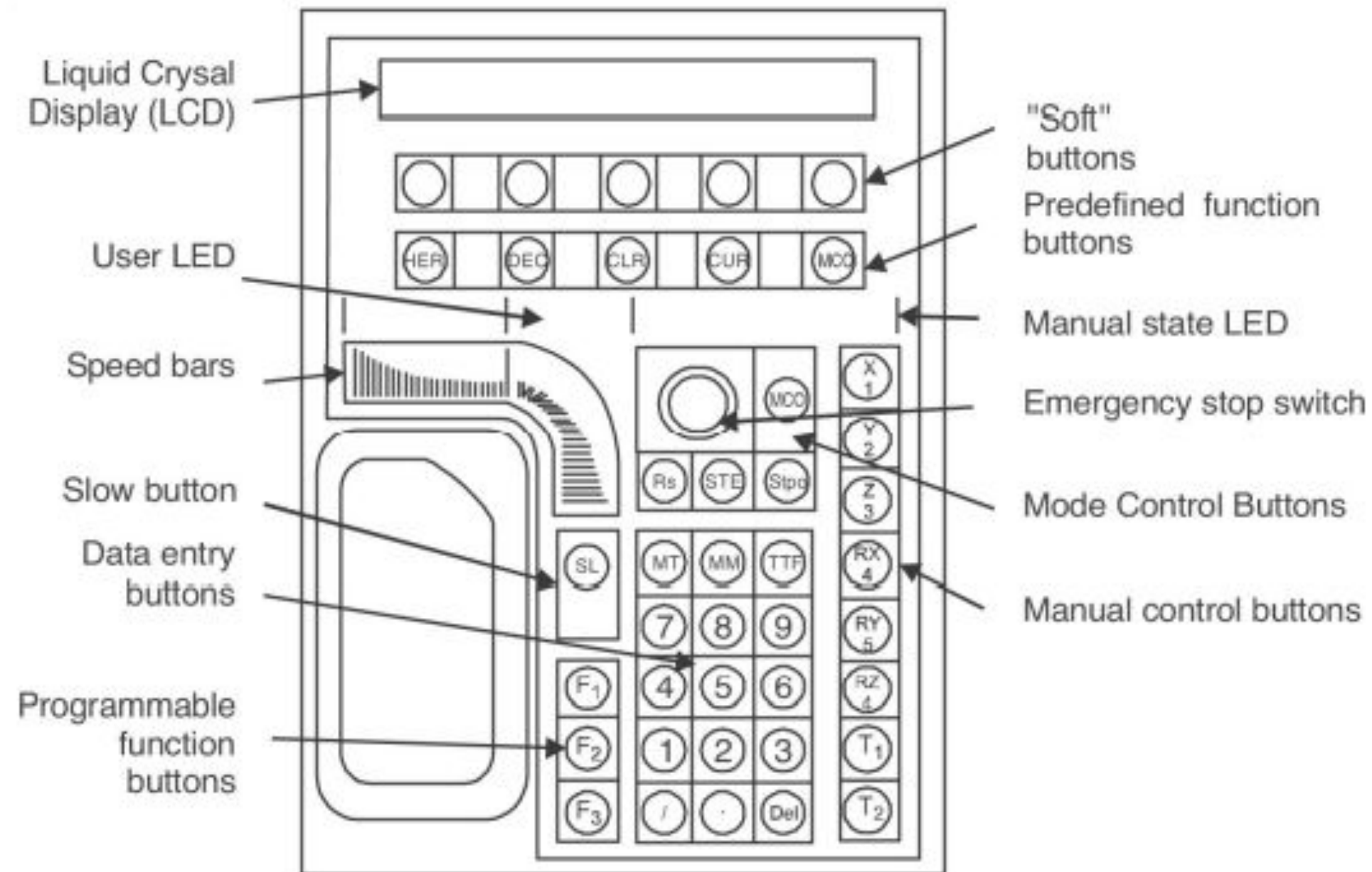
FIGURE 16.2 Teach Pendant.
