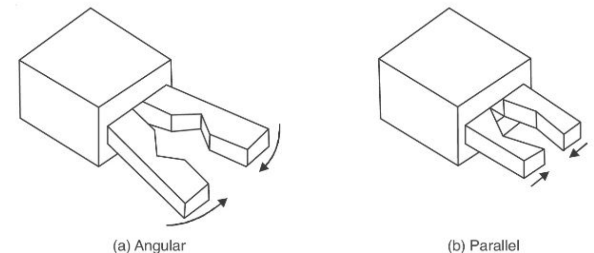
FIGURE 15.4 Angular and Parallel Grippers.
