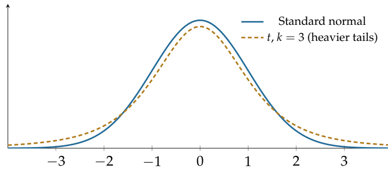
Figure 3.2: The t distribution (dashed) has heavier tails than the standard normal (solid). As k \rightarrow \infty the t distribution approaches the standard normal.
