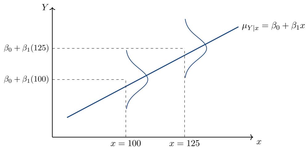
Figure 1.1: The true regression line is a line of mean values. At each x there is a distribution of Y with the same variance \sigma^2 .
