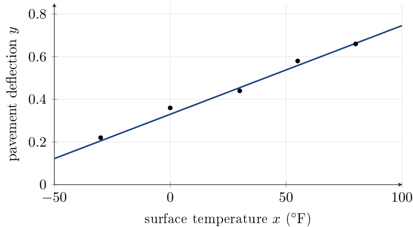
Figure 6.1: Fitted regression line \hat{y} = 0.32999 + 0.00416x for the pavement deflection data (illustrative points shown).
