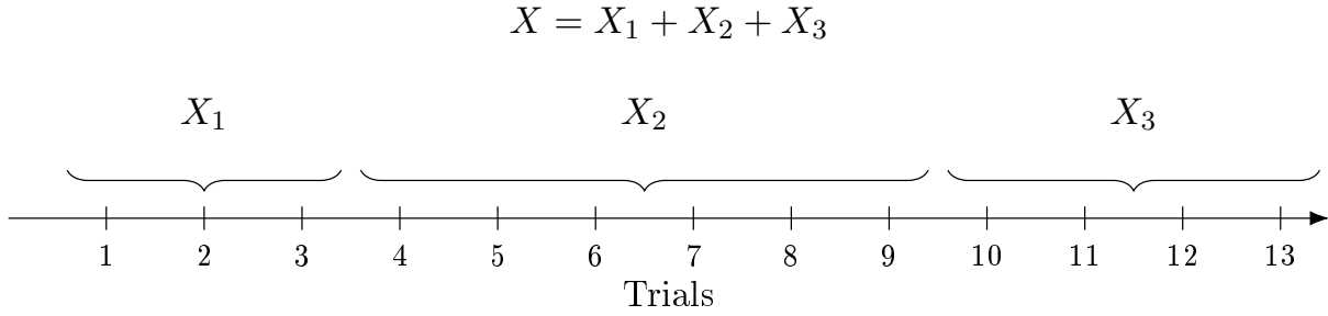
Figure 1.1: A negative binomial random variable ( r = 3 ) represented as the sum of three independent geometric random variables.
