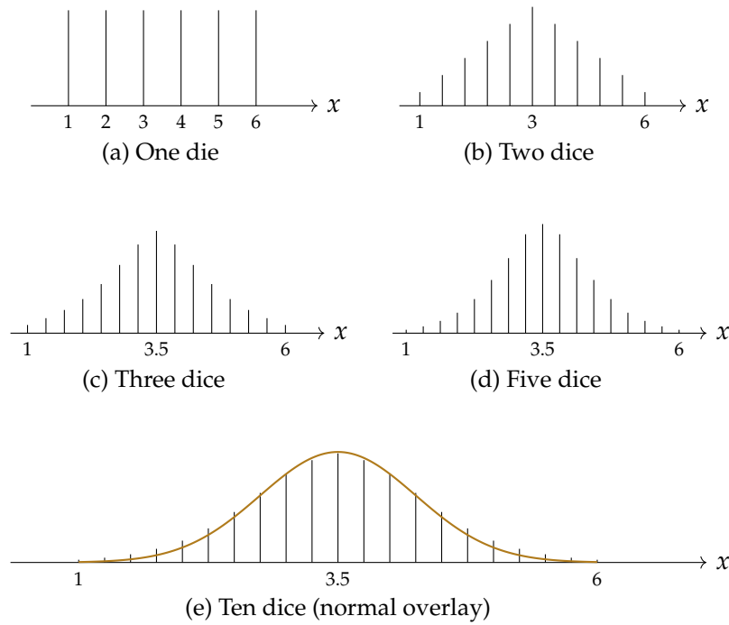
Figure 1.1: The distribution of the average score obtained when tossing n = 1, 2, 3, 5 and 10 dice. As n grows, the sampling distribution of the average approaches the normal shape.
