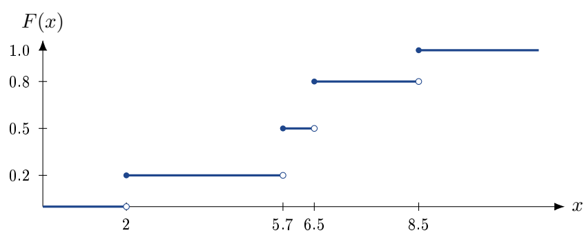
Figure 3.1: Step-function cumulative distribution function F(x) ; the jump heights give the probability mass function.
