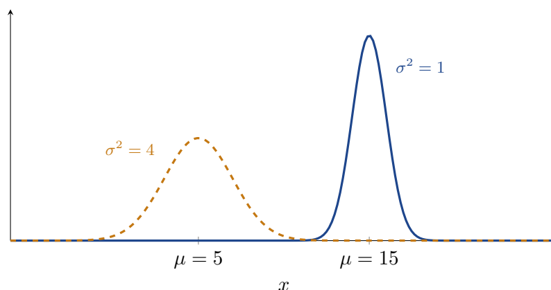
Figure 6.1: Normal densities with different means and variances. The mean locates the centre; the variance controls the spread.
