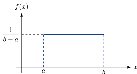
Figure 5.1: The continuous uniform probability density function on [a, b] .
