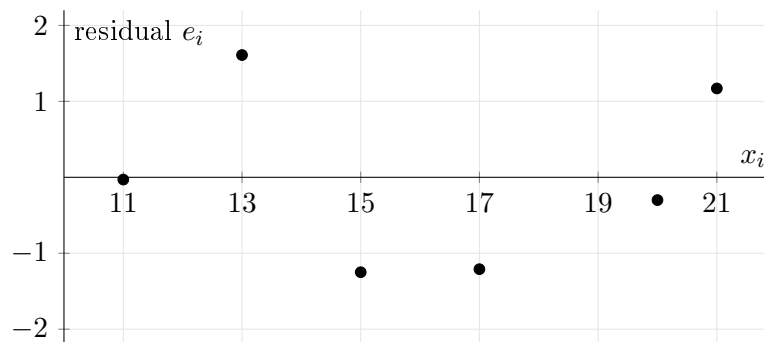
Figure 6.4: Residual plot. The scatter is sufficiently random; the sample size is small.
