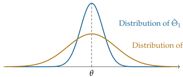
Figure 1.2: Two unbiased estimators of \theta . Both distributions are centred at the true value \theta , but \hat{\theta}_1 has the smaller variance and is therefore preferred.
