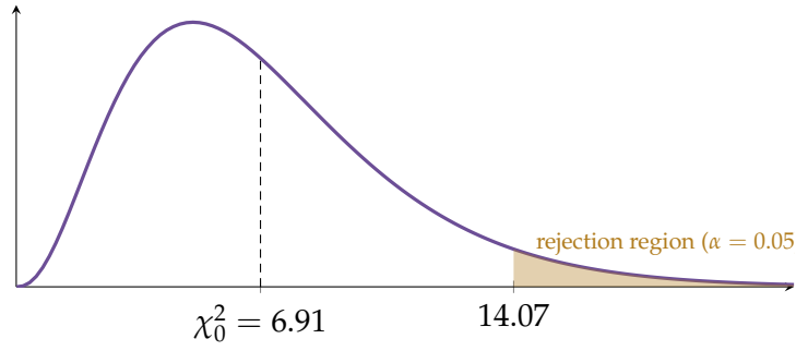
Figure 3.3: Chi-square density with 7 degrees of freedom. The observed statistic \chi_0^2 = 6.91 falls well short of the critical value 14.07, so H_0 is not rejected.
