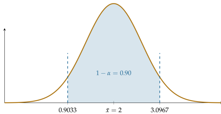
Figure 3.1: The 90% confidence interval 0.9033 \leq \mu \leq 3.0967 centred at \bar{x} = 2 , shown on the sampling distribution of the mean.
