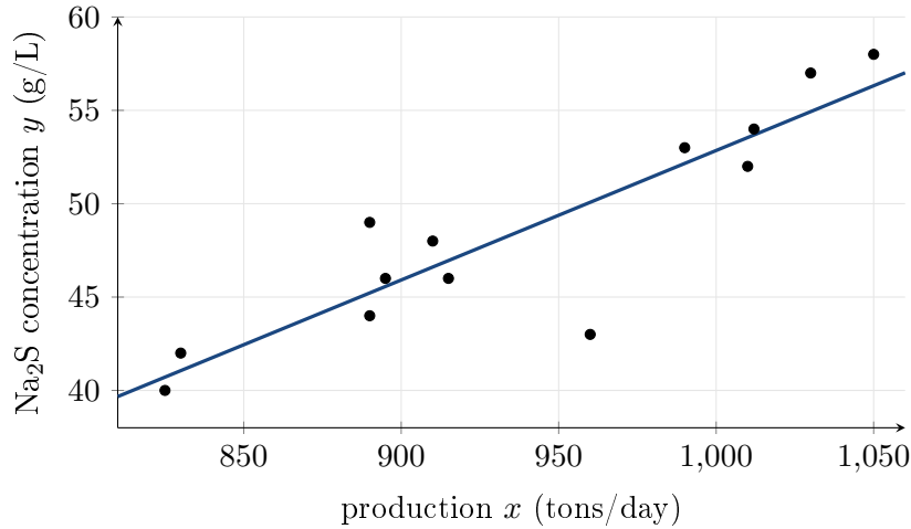
Figure 6.3: Scatter diagram of green liquor data with fitted line \hat{y} = -16.51 + 0.06936x .
