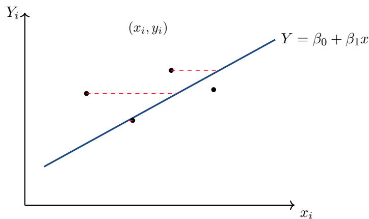
Figure 5.2: Reverse regression: horizontal deviations are minimized.
