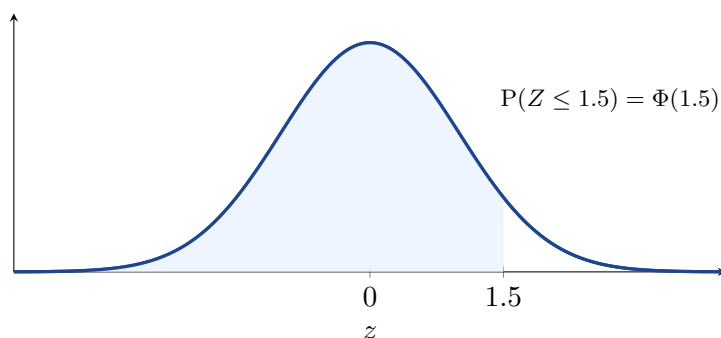
Figure 6.2: The standard normal density; the shaded area to the left of z = 1.5 is \Phi(1.5) .
