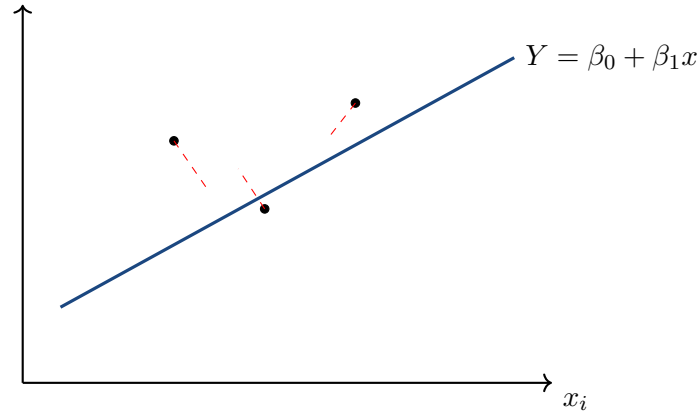
Figure 5.3: Major axis (orthogonal) regression: perpendicular distances are minimized.
