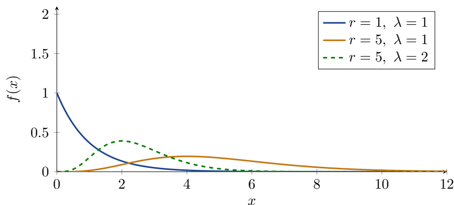
Figure 9.1: Erlang probability density functions for selected r and \lambda .
