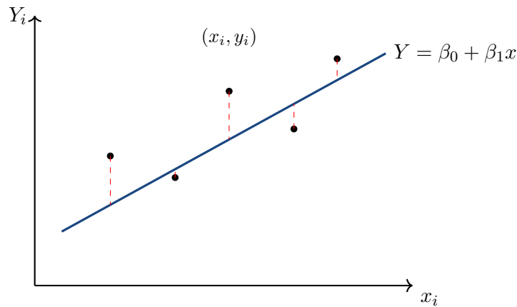
Figure 5.1: When the vertical differences between the observations and the line in the scatter diagram are considered and their sum of squares is minimized, the method is direct regression .
