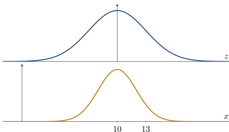
Figure 6.3: Standardizing a normal random variable: the transformation z = (x - \mu)/\sigma maps X \sim N(\mu, \sigma^2) onto the standard normal scale.
