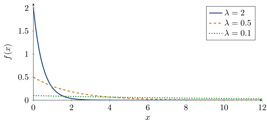
Figure 8.1: Exponential probability density functions for selected values of \lambda .
