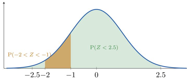
Figure 6.4: Standard-normal areas for the cement-strength problem: part (a) shaded light, part (b) shaded dark.
