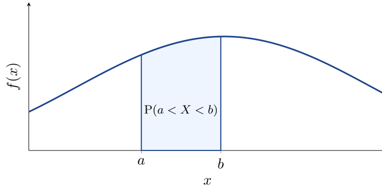
Figure 4.1: The probability that X lies between a and b is the shaded area under the density curve.
