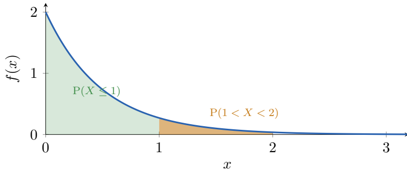
Figure 8.2: Exponential density f(x) = 2e^{-2x} with the areas for parts (c) and (d) shaded.
