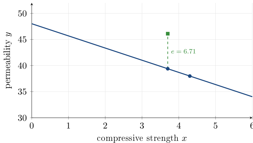
Figure 6.2: Fitted line \hat{y} = 48.013 - 2.3298x ; the residual at x = 3.7 is the dashed segment.
