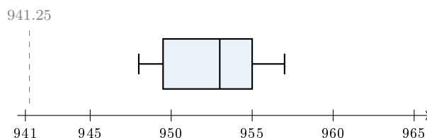
Figure 4.6: Box plot of the furnace-temperature data. No points fall beyond the fences, so there are no outliers.
