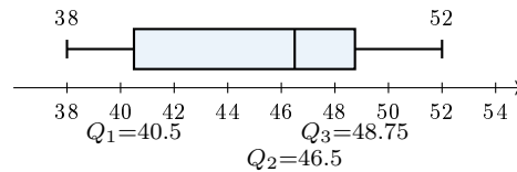
Figure 4.7: Box plot for the ten-point data set of Problem 4.
