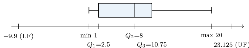
Figure 4.9: Box plot for Problem 6. Since both the minimum and maximum lie within the fences, there are no outliers .
