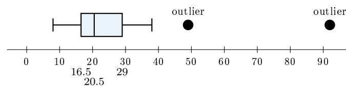
Figure 4.8: Box plot for Problem 5. Interpretation: the data set is unsymmetric; the middle 50% of the data lie between 16.5 and 29. The value 49 is a suspected outlier, and 92 is an outlier.
