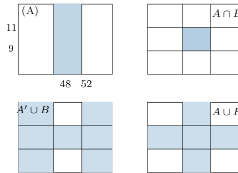
Figure 6.2: Shaded Venn-style regions for the length-width events: A , A \cap B , A' \cup B , and A \cup B , where A is the vertical band 48 < X < 52 and B is the horizontal band 9 < Y < 11 .
