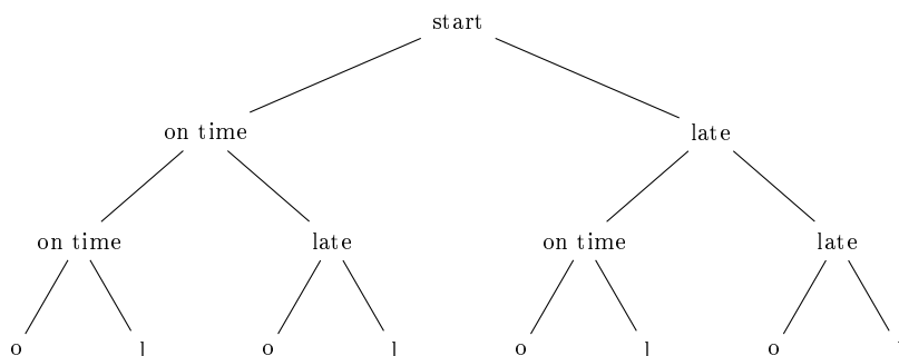
Figure 5.2: Tree diagram for the classification of 3 messages, each “on time” (o) or “late” (l), giving 2^3 = 8 branches.
