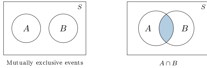
Figure 5.3: Venn diagrams: mutually exclusive events (left) and the intersection A \cap B of two overlapping events (right).
