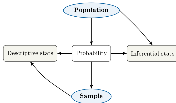
Figure 2.1: Probability links a population to its samples and connects descriptive and inferential statistics. Knowledge of the population, processed through probability, yields expected properties of a sample; sample data, processed through probability, support inferences about the population.
