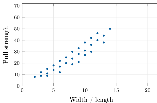
Figure 4.1: A scatter plot. Scatter plots show the region of the plane where data points fall, as well as the data density associated with that region. They also suggest possible association between the variables. Unlike dot plots, scatter plots can be used for large data sets as well.
