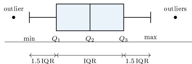
Figure 4.5: Anatomy of a box plot. The box spans the interquartile range from Q_1 to Q_3 , the central line marks the median Q_2 , and whiskers reach the most extreme non-outlier values. Points beyond 1.5 IQR of the quartiles are outliers.
