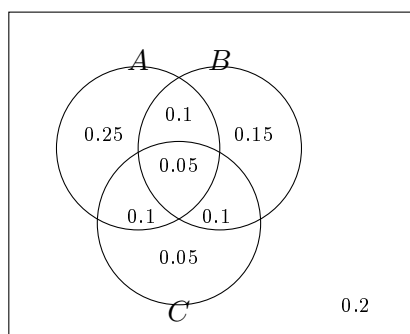
Figure 6.3: Venn diagram for the customer-order problem, with probabilities assigned to each disjoint region.
