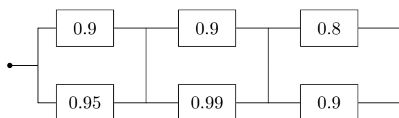
Figure 7.1: Three parallel blocks connected in series.
