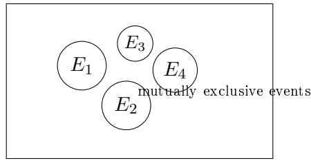
Figure 6.1: A collection of mutually exclusive events partitioning part of the sample space.
