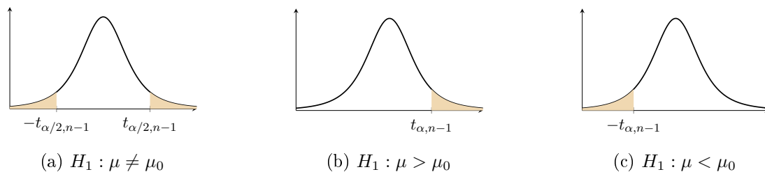
Figure 4.2: The reference t_{n-1} distribution with critical regions (shaded) for the three alternative hypotheses.
