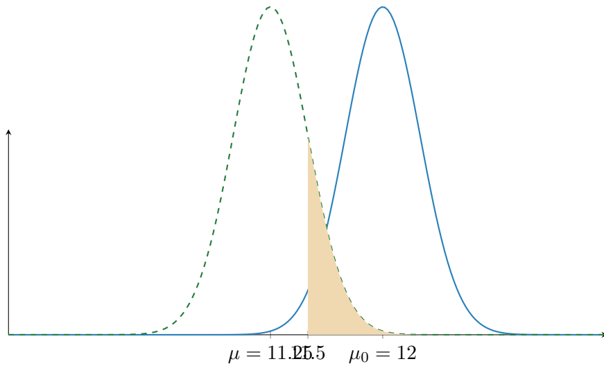
Figure 2.1: Type II error ( \beta , shaded) when the true mean is 11.25: the null curve is centred at \mu_0 = 12 and the true curve at \mu = 11.25 .
