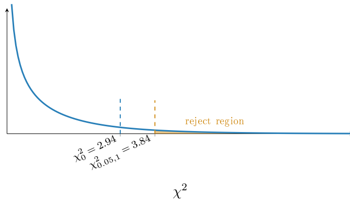
Figure 5.1: Chi-square distribution with 1 degree of freedom. The statistic \chi_0^2 = 2.94 falls left of the critical value 3.84, so H_0 is not rejected.
