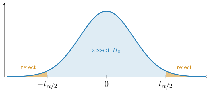
Figure 4.3: Two-sided rejection region for the t -test: reject H_0 when |t_0| > t_{\alpha/2, n-1} .
