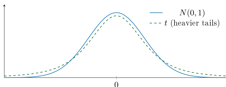
Figure 4.1: The t distribution compared to the standard normal: same symmetric, unimodal shape but heavier tails.
