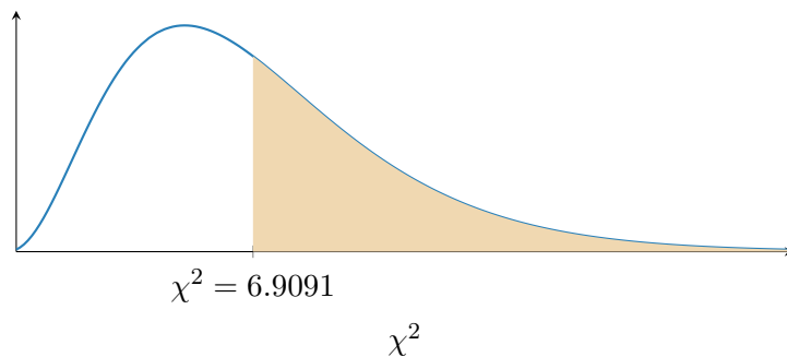
Figure 6.1: Chi-square distribution with 7 degrees of freedom; the shaded upper tail beyond \chi^2 = 6.9091 gives the P -value ( 0.4 < P < 0.5 ).
