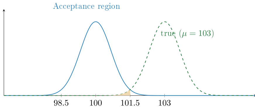
Figure 2.2: Type II error ( \beta , shaded) when the true mean is 103; the acceptance region [98.5, 101.5] is set under the null curve centred at 100.
