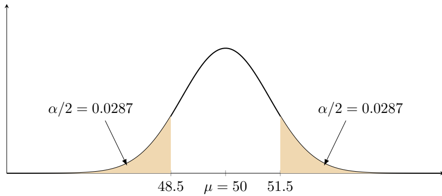
Figure 1.1: Critical region for H_0 : \mu = 50 versus H_1 : \mu \neq 50 with n = 10 .
