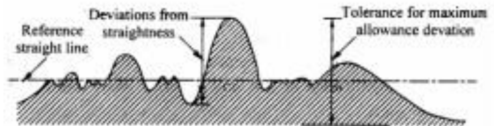
Fig 3.27 Straightness Measurement
