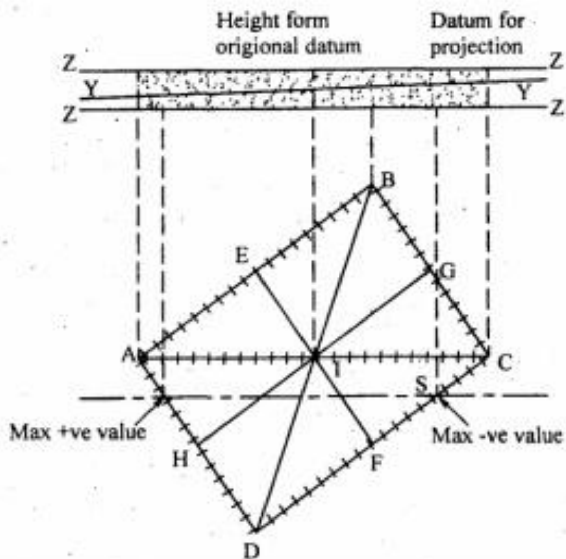
Fig 3.29 Flatness Testing
