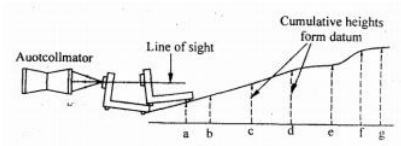
Fig 3.28 Straightness using Auto-Collimator
