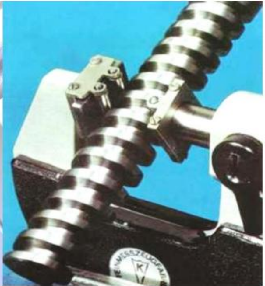
Principle of three-wire method
