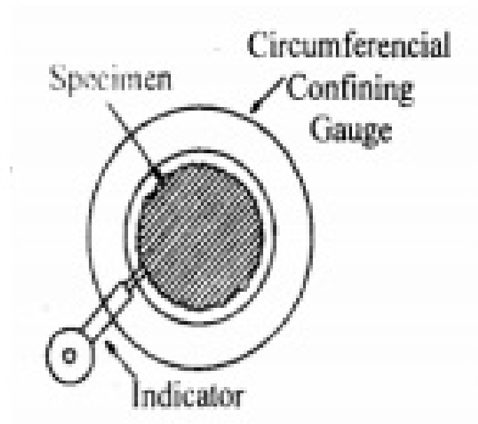
Fig 3.30 Confining Gauge
