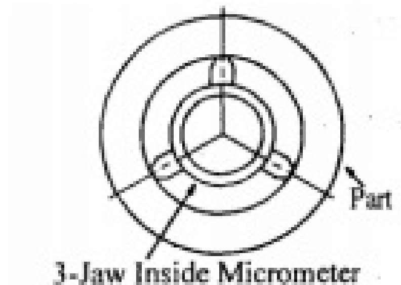
Fig 3.32 Three Point Probe
