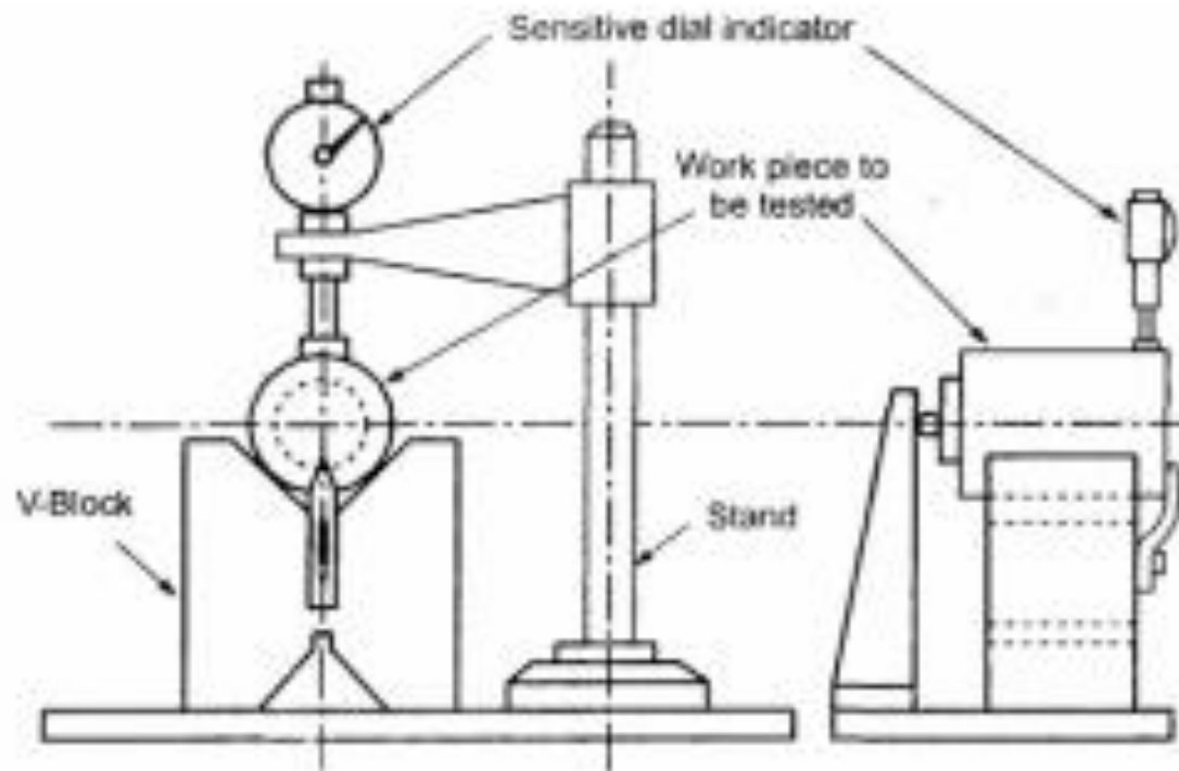
Fig 3.31 V-Block
