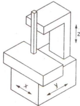
Figure 8.3 : Column Structure
