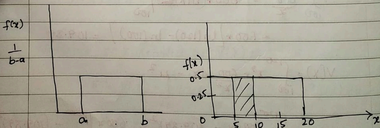
Continuous UNIFORM PDF
