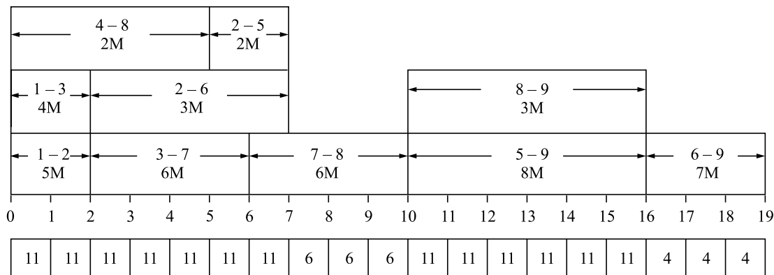
Fig. 13.40 Loading Chart
