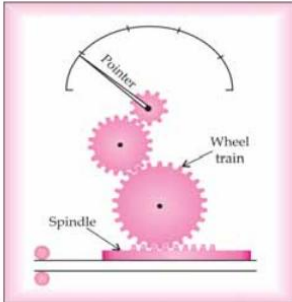
Dial Indicator
