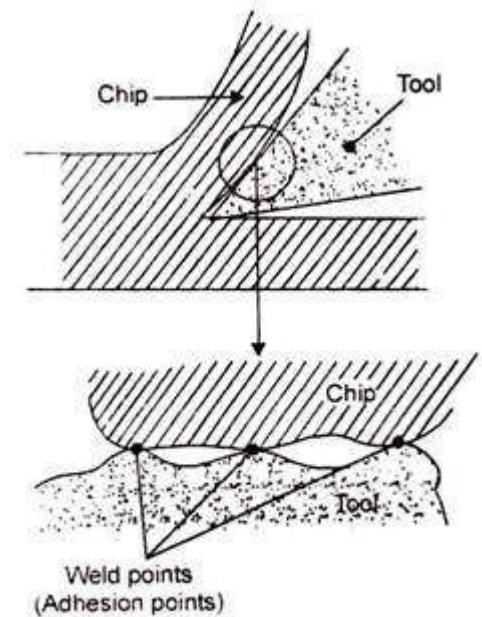
Fig. 9.19. Adhesion Wear.
