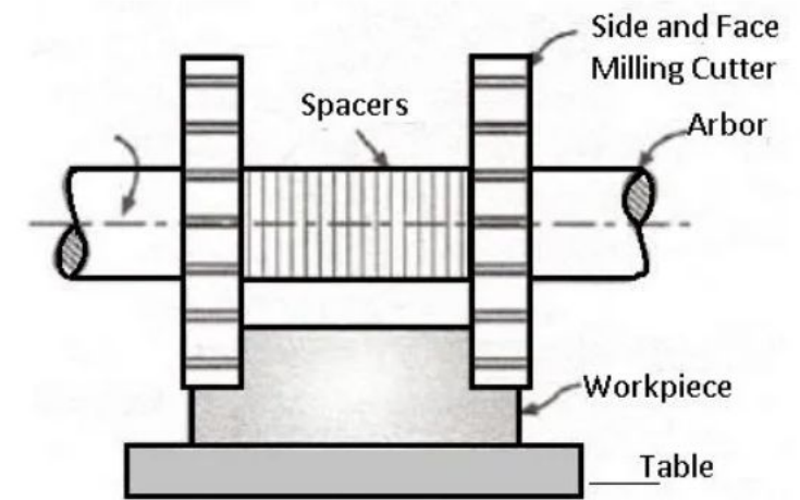
Straddle Milling Operation
