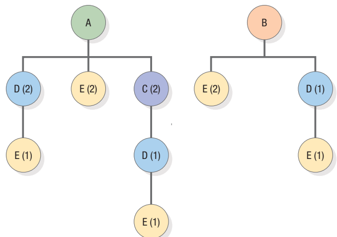
▼ FIGURE 16.42 BOMs for Products A and B
