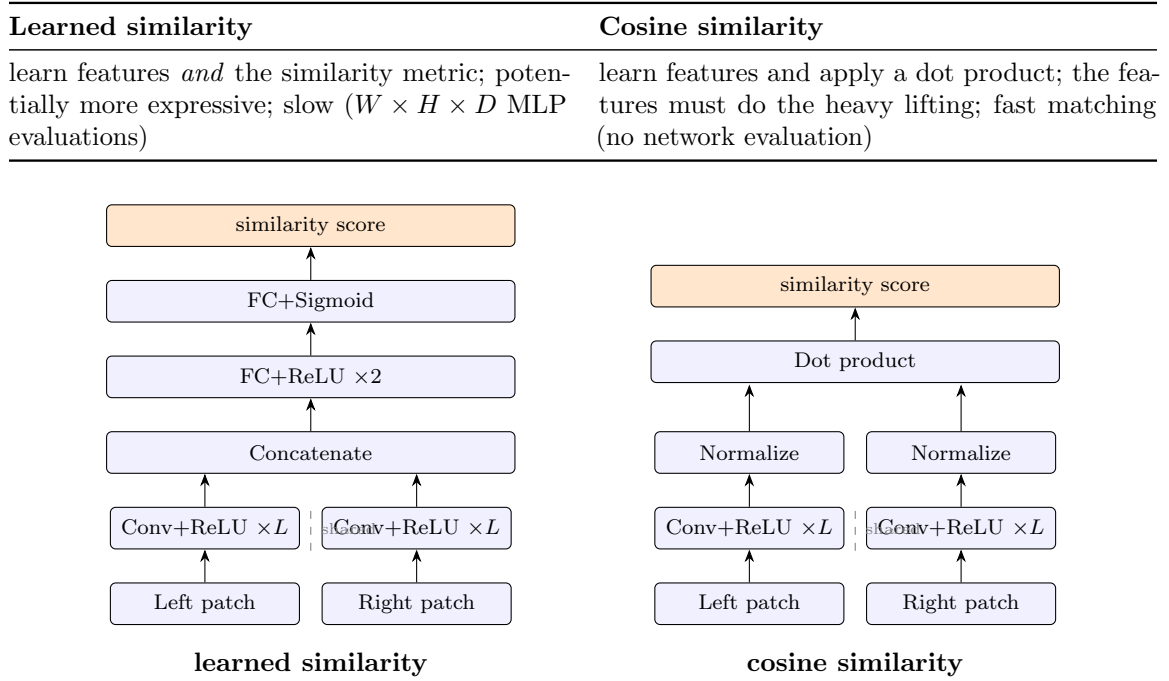
Figure 20: The two Siamese stereo architectures of Zbontar and LeCun (redrawn from slide 24; layer counts are schematic). Both towers share weights.
