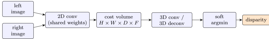
Figure 28: GC-Net pipeline (redrawn from slide 31).
