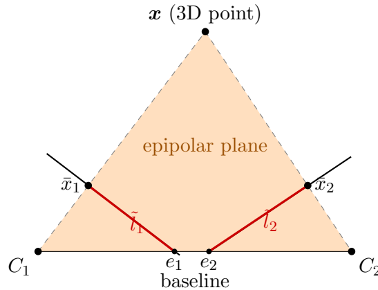
Figure 3: Epipolar geometry (redrawn from slide 7). The camera centres and the 3D point span the epipolar plane; it cuts each image plane in an epipolar line, and the baseline pierces the image planes at the epipoles.
