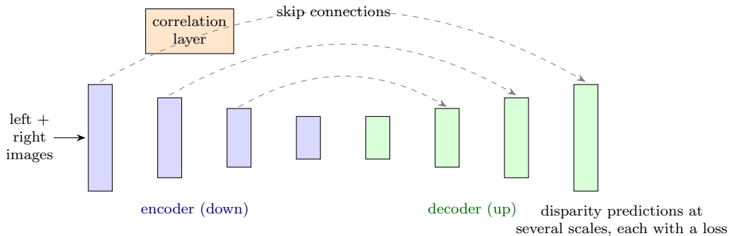
Figure 26: Schematic of a DispNet-style encoder–decoder with skip connections (new schematic, not a reproduction of the slide’s network figure).
