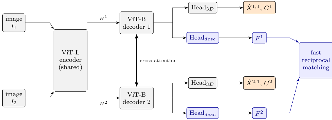
Figure 32: DUS3R/MASt3R architecture (redrawn from slides 36 and 39; blue = MASt3R additions).
