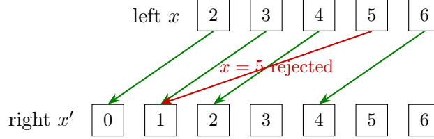
Figure 17: Toy left-to-right matches from the example (new figure). Two left pixels landing on the same right pixel flags an inconsistency.
