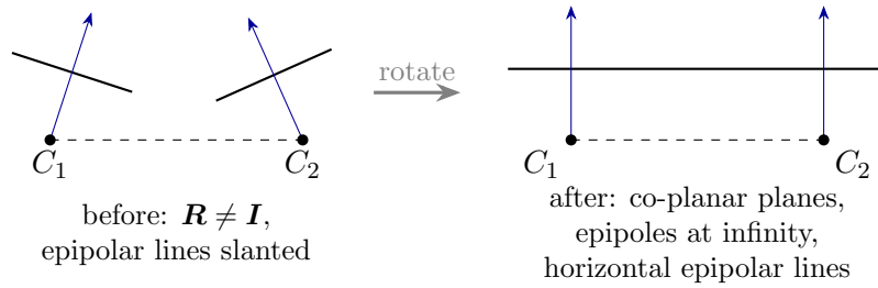
Figure 4: Rectification as a pure rotation of each camera (top view; blue arrows are optical axes). After the rotation both image planes are the same plane, parallel to the baseline.
