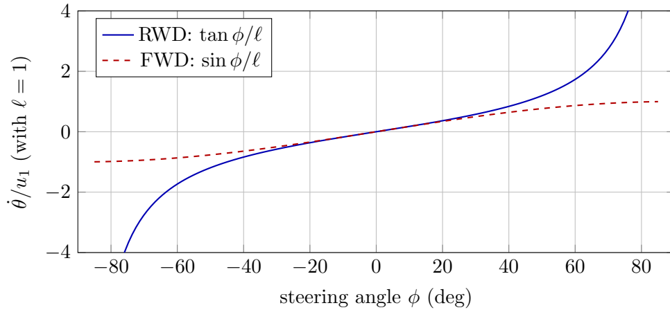
Figure 53: Rotation rate per unit of drive speed: it blows up at \phi = \pm\pi/2 for the rear-wheel-drive model but stays bounded for the front-wheel-drive one.
