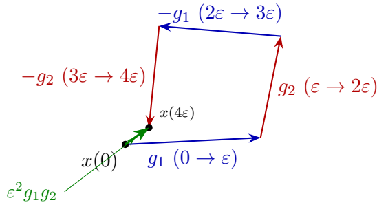
Figure 50: The four legs of the manoeuvre almost close a loop; the gap is the displacement \varepsilon^2 g_1 g_2(x_0) (schematic, exaggerated).
