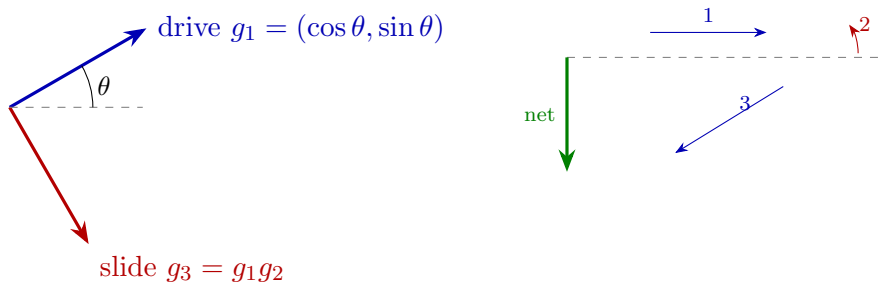
Figure 51: Left: drive and slide vectors of the unicycle. Right: LB manoeuvre (1 forward, 2 rotate, 3 backward, then rotate back): the net displacement is sideways (angles exaggerated).
