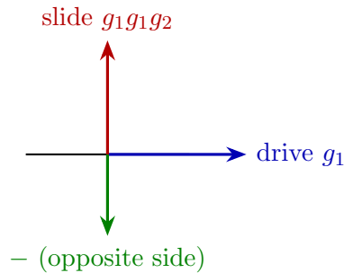
Figure 52: Bicycle at \theta = 0 : the second-order bracket g_1 g_1 g_2 \propto (-\sin \theta, \cos \theta, 0, 0) is the sliding direction, perpendicular to the heading.
