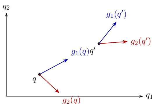
Figure 38: The basis vectors g_i(q) are vector fields: at each configuration they give (generally different) admissible directions.
