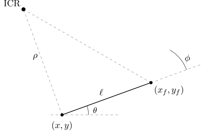
Figure 46: Bicycle geometry. The axes of the two wheels (perpendicular to the rolling directions) meet at the instantaneous centre of rotation (ICR); the whole robot rotates instantaneously about it, with turning radius \rho = \ell / \tan \phi .
