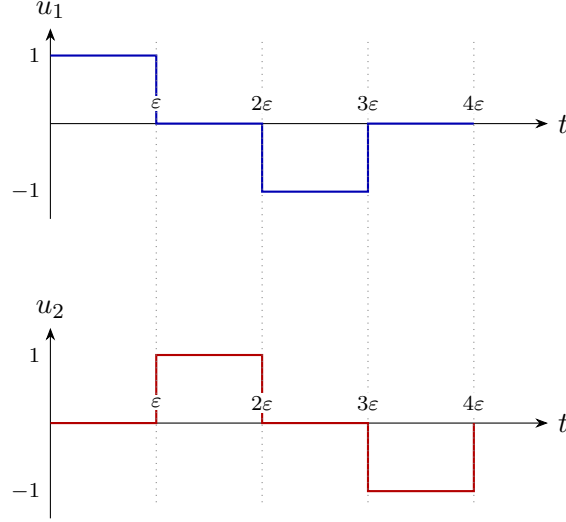
Figure 49: Control sequence of Algorithm 30.1: forward g_1 , forward g_2 , backward g_1 , backward g_2 .
