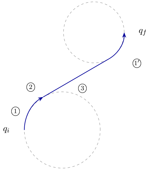
Figure 48: Schematic universal manoeuvre (arc around an ICR, straight line, arc). The numbers refer to the steps of the algorithm; 1' is the final arc that matches the target heading.
