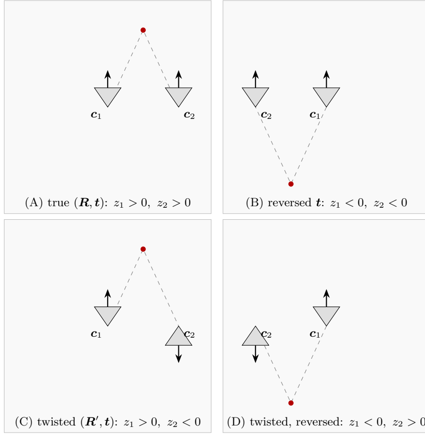
Figure 122: Schematic of the four candidate poses (after slide 27; in 2D, cameras drawn as triangles with an arrow along the viewing direction, red dot: reconstructed point, dashed: reconstructed rays). Only panel A has the point in front of both cameras.
