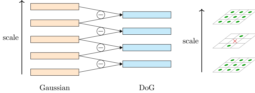
Figure 114: Left: first octave of the Gaussian scale space and the DoG images obtained by subtracting neighbouring scales. Right: a candidate (red cross) is kept only if it is larger or smaller than all its 26 neighbours in space and scale (green).
