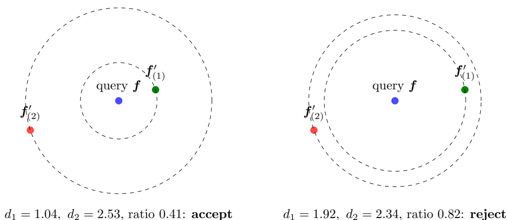
Figure 116: Toy example in a 2D descriptor space. If the best match is not clearly better than the runner-up, the match is ambiguous.
