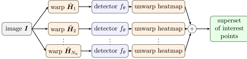
Figure 118: Homographic Adaptation (redrawn from slide 18): detect on warped copies, un-warp, average, and extract the pseudo-ground-truth points.
