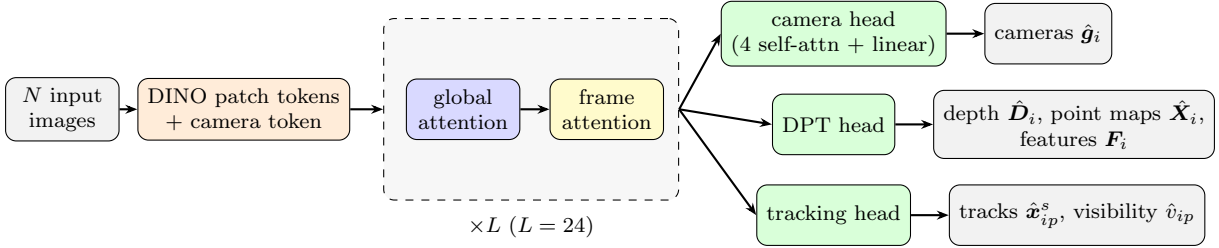
Figure 131: VGGT architecture (redrawn and simplified from slide 60).
