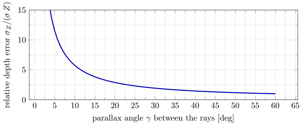
Figure 125: Original illustration of the trade-off. For a point at distance Z seen under angular noise \sigma per ray, the depth error is, to first order, \sigma_Z \approx \sigma Z / (2 \sin(\gamma/2)) \approx \sigma Z / \gamma (small \gamma ). Below about 5^\circ the error explodes; above about 30^\circ it is flat, but matching becomes hard.
