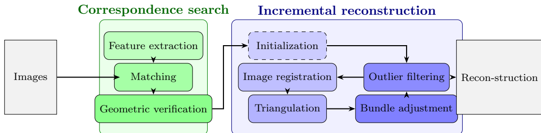
Figure 129: Incremental SfM pipeline of COLMAP (redrawn from slide 45). The registration–triangulation–filtering–bundle–adjustment loop runs once per added image.
