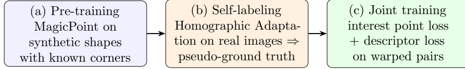
Figure 117: The three SuperPoint training stages (slide 16).
