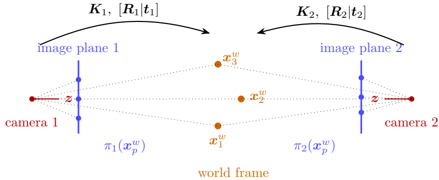
Figure 126: The bundle adjustment setup (slide 39): the 3D points are projected into both cameras by \pi_i . With the \mathbf{K}_i fixed, bundle adjustment optimizes the poses \mathcal{T} and the points \mathcal{X}_w jointly.
