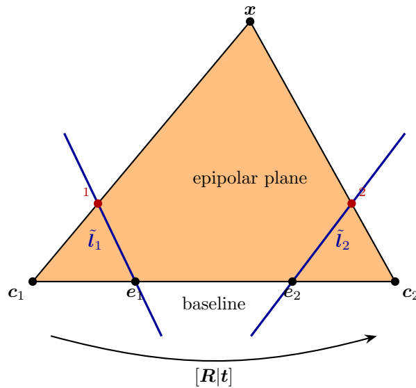
Figure 121: Epipolar geometry (redrawn from slide 22). The image planes are drawn edge-on: their intersection with the epipolar plane is the epipolar line.
