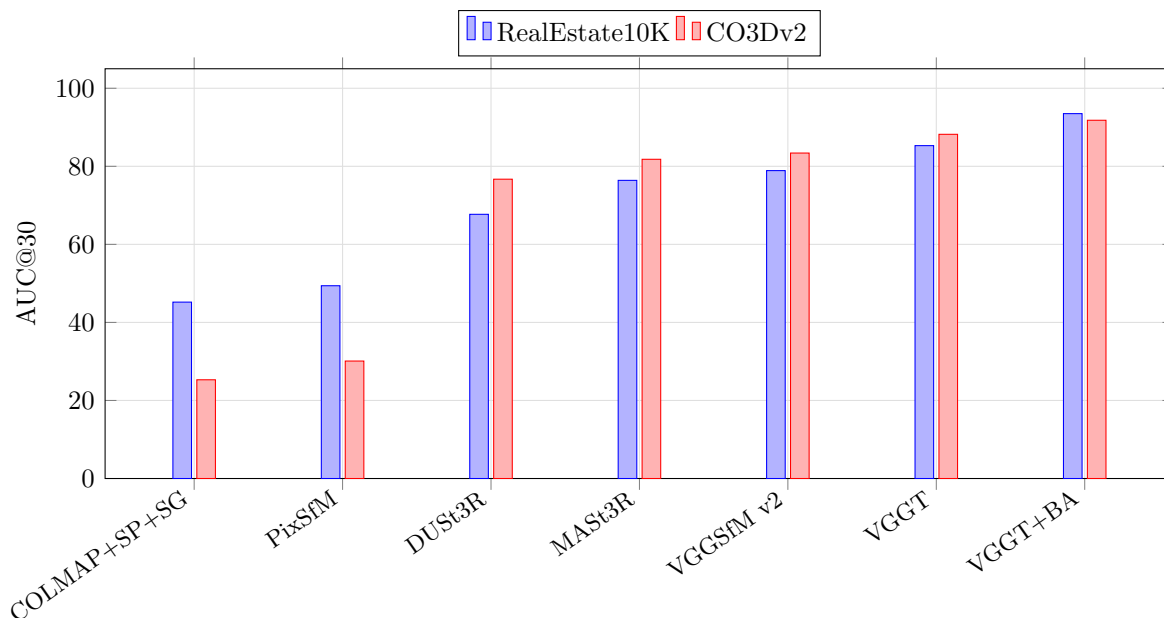
Figure 132: Camera pose accuracy of classical, learned two-view, and feed-forward methods (data of the table on slide 63; ten random frames per scene). The jump from the classical pipeline to learned methods is largest in the sparse regime, and bundle adjustment on top of VGGT adds the final gain.
