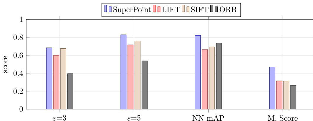
Figure 120: Selected HPatches metrics from the table (higher is better).
