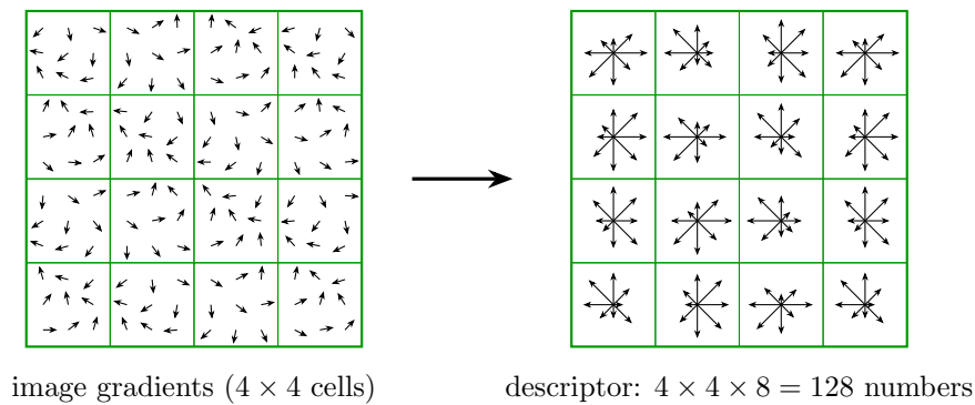
Figure 115: Schematic of the SIFT descriptor: the gradients around the keypoint (after rotating to the dominant orientation) are pooled into an orientation histogram with 8 bins per cell; 4 x 4 cells give a 128D vector.
