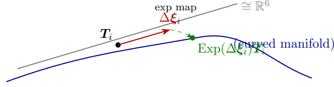
Figure 127: Local update on a curved space: take a step \Delta\xi_i in the flat tangent space, then map it back onto the group with the exponential map (schematic).
