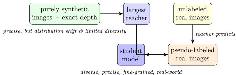
Figure 62: Depth Anything V2 pipeline (redrawn from slide 34).
