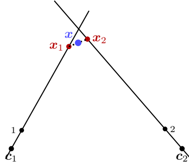
Figure 123: Two noisy rays do not intersect; \mathbf{x}_1, \mathbf{x}_2 are their closest points and \mathbf{x} their midpoint (slide 32).
