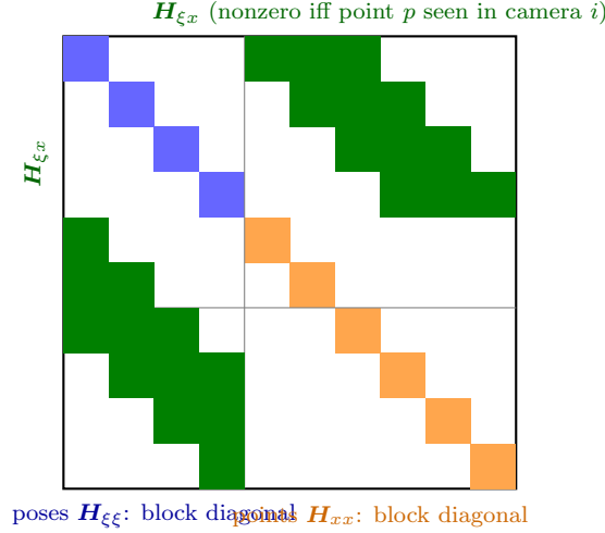
Figure 128: Arrowhead sparsity of the BA Hessian for N = 4 cameras and P = 6 points (original illustration). Cameras and points interact only if they share an observation. Eliminating the points (orange) leaves a small 4 \times 4 -block reduced camera system.
