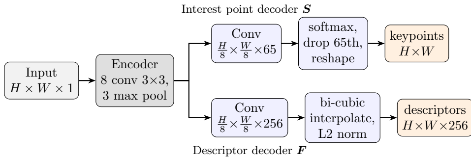
Figure 119: SuperPoint architecture (redrawn from slide 19).
