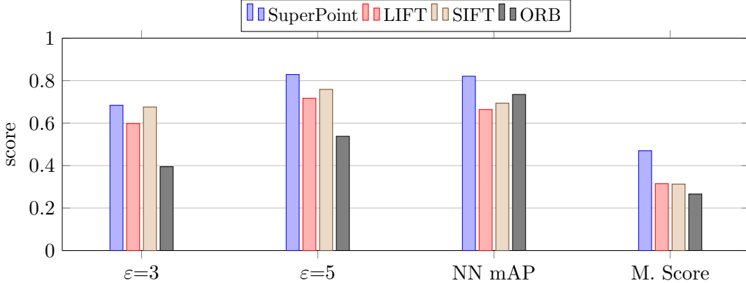
Figure 8: Selected HPatches metrics from the table (higher is better).
