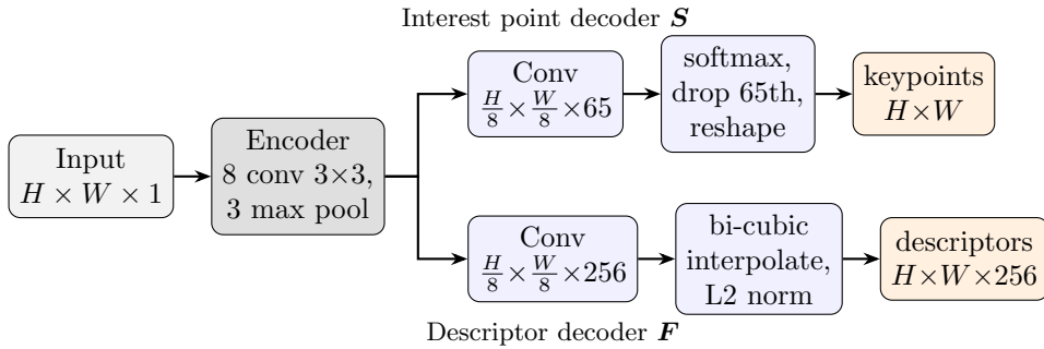
Figure 7: SuperPoint architecture (redrawn from slide 19).
