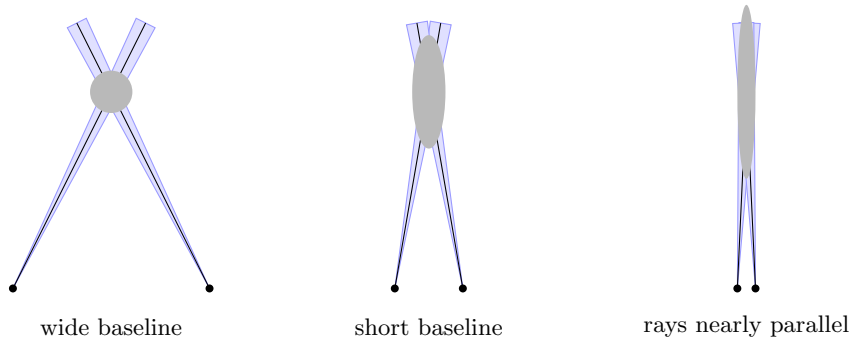
Figure 12: Schematic of triangulation uncertainty (after slide 35): the grey region is where the two noisy rays are consistent with the observations. It grows as the rays become parallel. The ellipses are drawn by hand, not computed.
