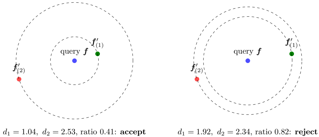
Figure 4: Toy example in a 2D descriptor space. If the best match is not clearly better than the runner-up, the match is ambiguous.
