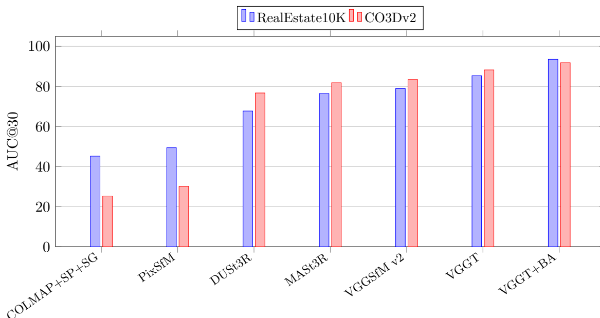
Figure 20: Camera pose accuracy of classical, learned two-view, and feed-forward methods (data of the table on slide 63; ten random frames per scene). The jump from the classical pipeline to learned methods is largest in the sparse regime, and bundle adjustment on top of VGGT adds the final gain.
