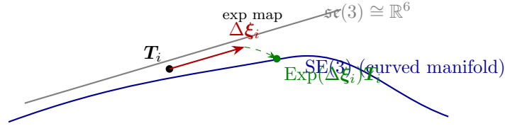
Figure 15: Local update on a curved space: take a step \Delta\xi_i in the flat tangent space, then map it back onto the group with the exponential map (schematic).
