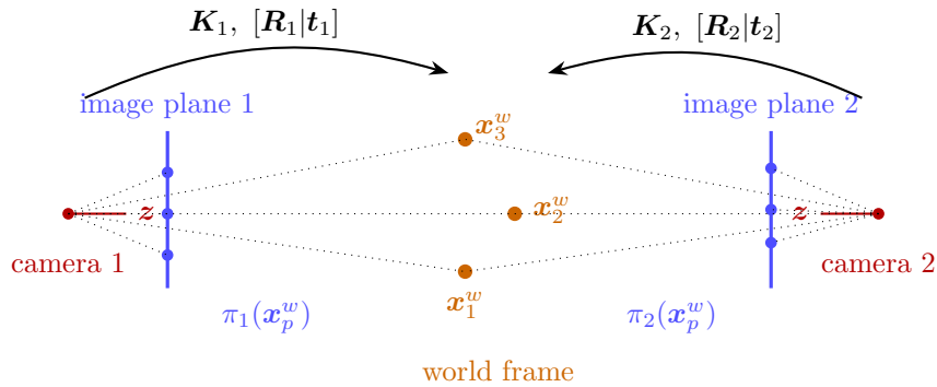
Figure 14: The bundle adjustment setup (slide 39): the 3D points are projected into both cameras by \pi_i . With the \mathbf{K}_i fixed, bundle adjustment optimizes the poses \mathcal{T} and the points \mathcal{X}_w jointly.
