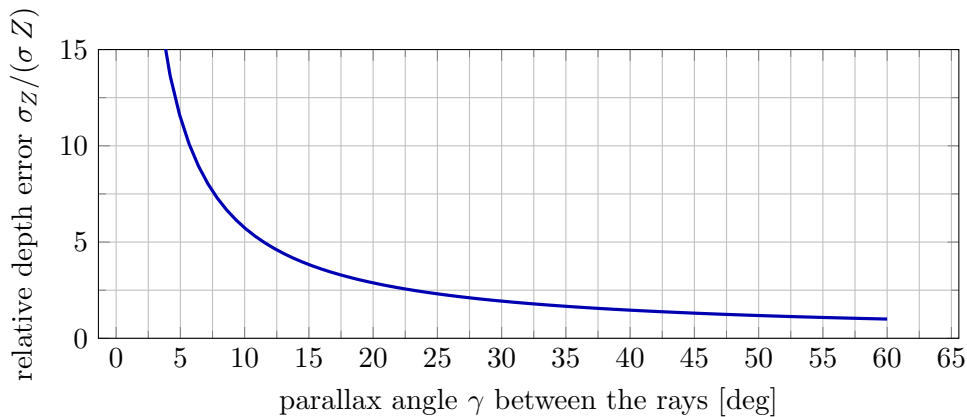
Figure 13: Original illustration of the trade-off. For a point at distance Z seen under angular noise \sigma per ray, the depth error is, to first order, \sigma_Z \approx \sigma Z / (2 \sin(\gamma/2)) \approx \sigma Z / \gamma (small \gamma ). Below about 5^\circ the error explodes; above about 30^\circ it is flat, but matching becomes hard.
