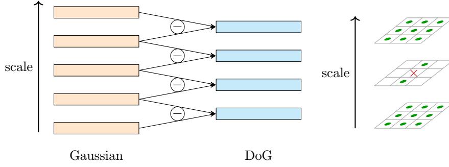
Figure 2: Left: first octave of the Gaussian scale space and the DoG images obtained by subtracting neighbouring scales. Right: a candidate (red cross) is kept only if it is larger or smaller than all its 26 neighbours in space and scale (green).
