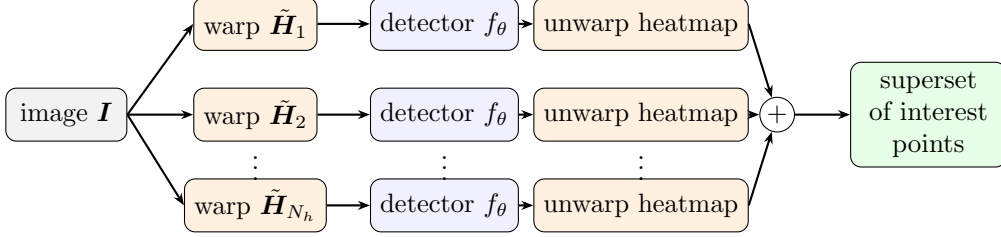
Figure 6: Homographic Adaptation (redrawn from slide 18): detect on warped copies, un-warp, average, and extract the pseudo-ground-truth points.
