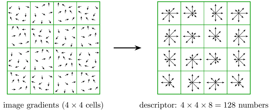
Figure 3: Schematic of the SIFT descriptor: the gradients around the keypoint (after rotating to the dominant orientation) are pooled into an orientation histogram with 8 bins per cell; 4 × 4 cells give a 128D vector.
