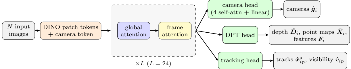
Figure 19: VGGT architecture (redrawn and simplified from slide 60).
