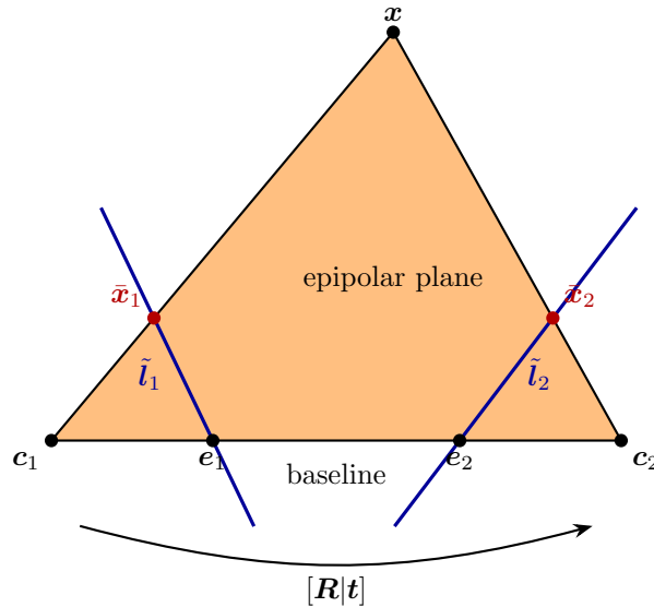
Figure 9: Epipolar geometry (redrawn from slide 22). The image planes are drawn edge-on: their intersection with the epipolar plane is the epipolar line.
