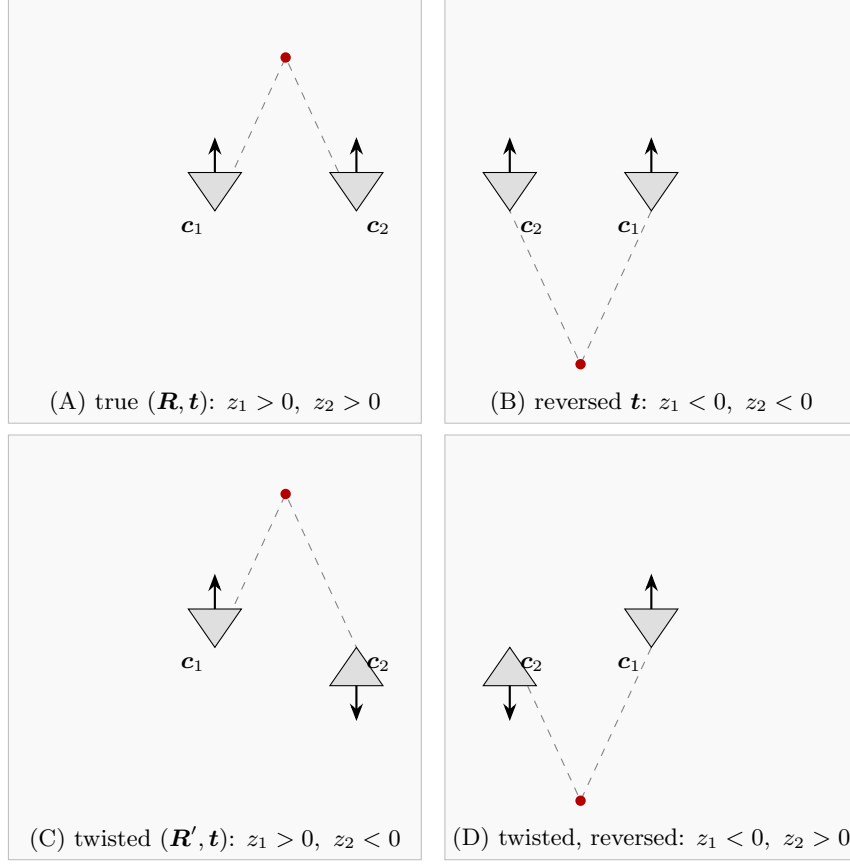
Figure 10: Schematic of the four candidate poses (after slide 27; in 2D, cameras drawn as triangles with an arrow along the viewing direction, red dot: reconstructed point, dashed: reconstructed rays). Only panel A has the point in front of both cameras.
