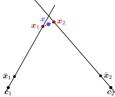
Figure 11: Two noisy rays do not intersect; \mathbf{x}_1, \mathbf{x}_2 are their closest points and \mathbf{x} their midpoint (slide 32).
