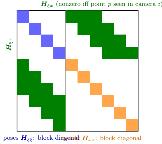
Figure 16: Arrowhead sparsity of the BA Hessian for N = 4 cameras and P = 6 points (original illustration). Cameras and points interact only if they share an observation. Eliminating the points (orange) leaves a small 4 \times 4 -block reduced camera system.
