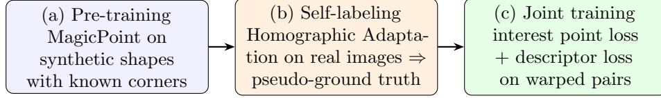
Figure 5: The three SuperPoint training stages (slide 16).
