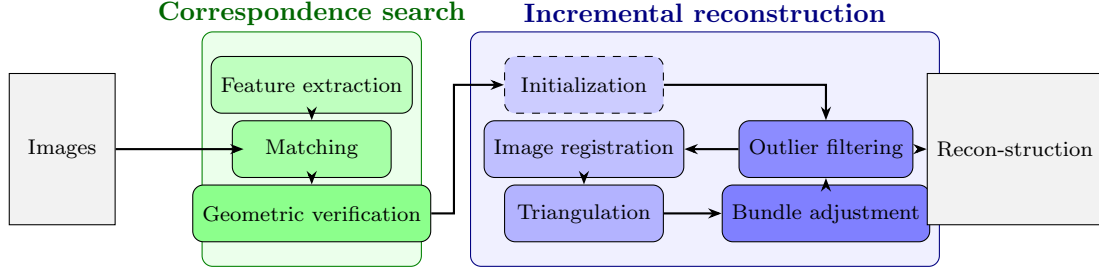
Figure 17: Incremental SfM pipeline of COLMAP (redrawn from slide 45). The registration–triangulation–filtering–bundle–adjustment loop runs once per added image.
