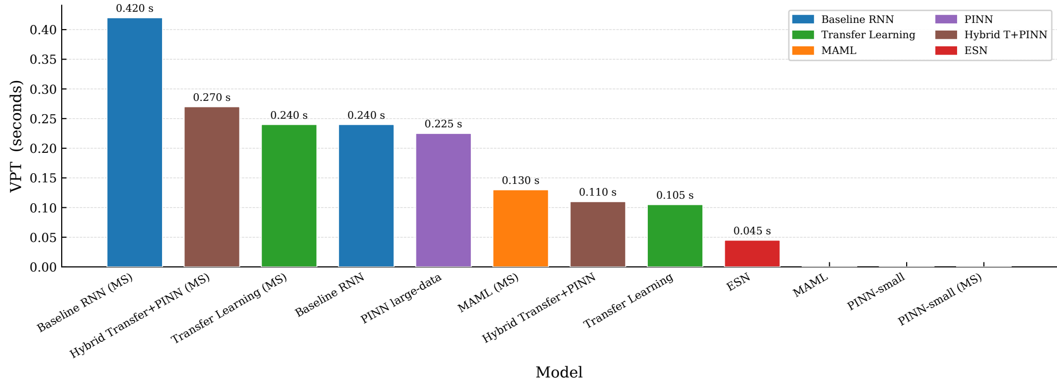
KS — Valid Prediction Time in Seconds ( \lambda_1 \approx 0.094 (L=36))
