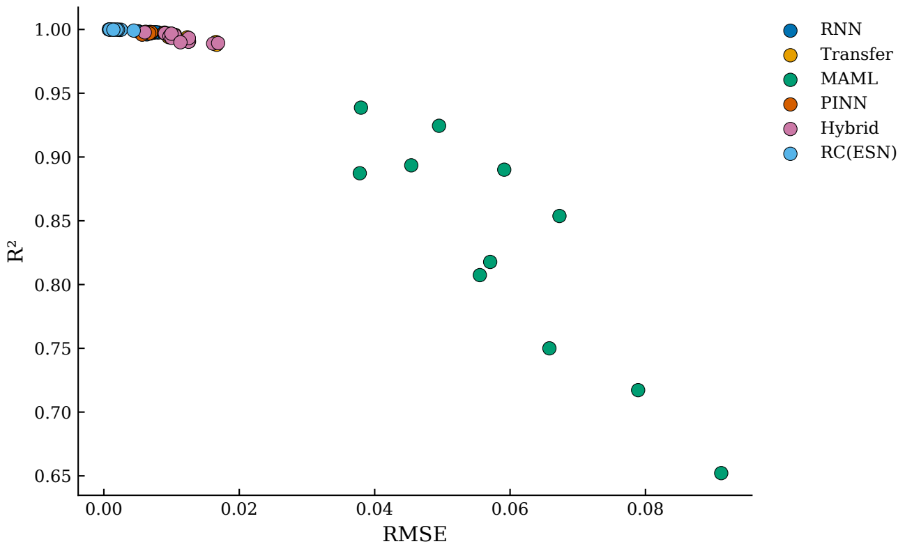
KS — RMSE vs R^2 : All Method \times IC (stable ICs)
