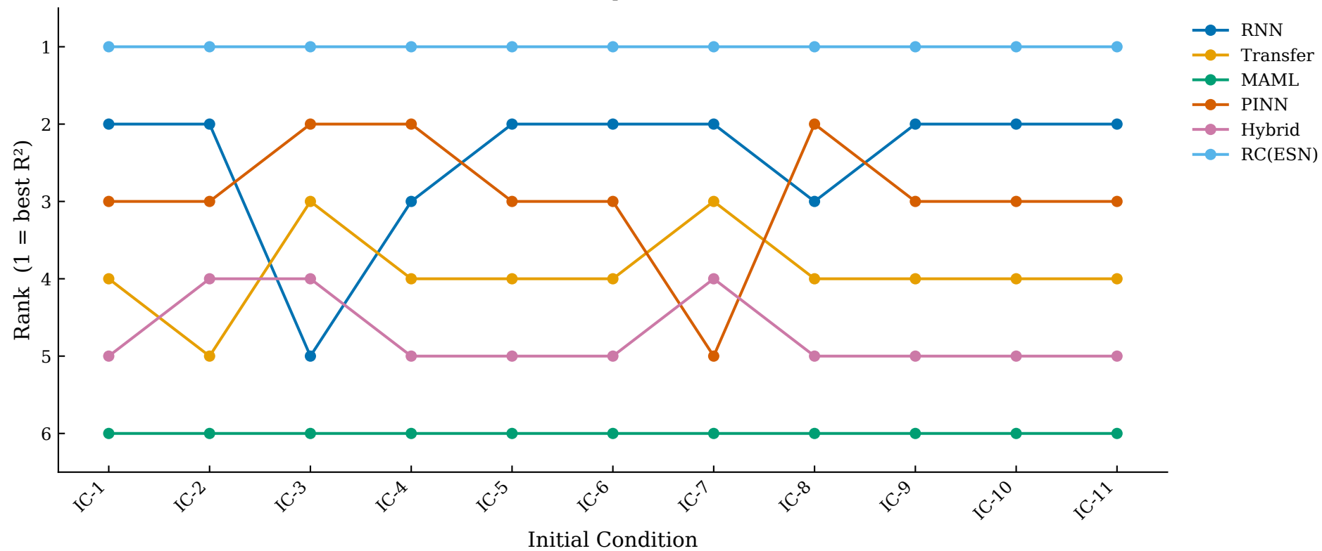
KS — Method Rank per Initial Condition
