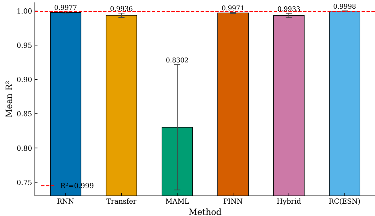
KS — Mean R^2 per Method (stable ICs) (error bars = std across ICs)
