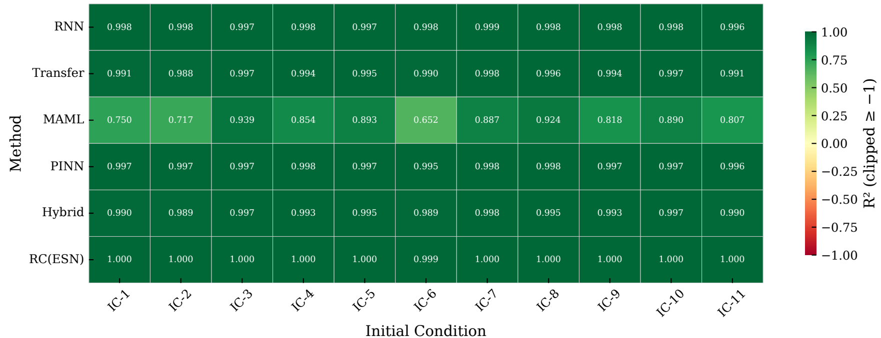
KS — R 2 Heatmap: Method × IC
