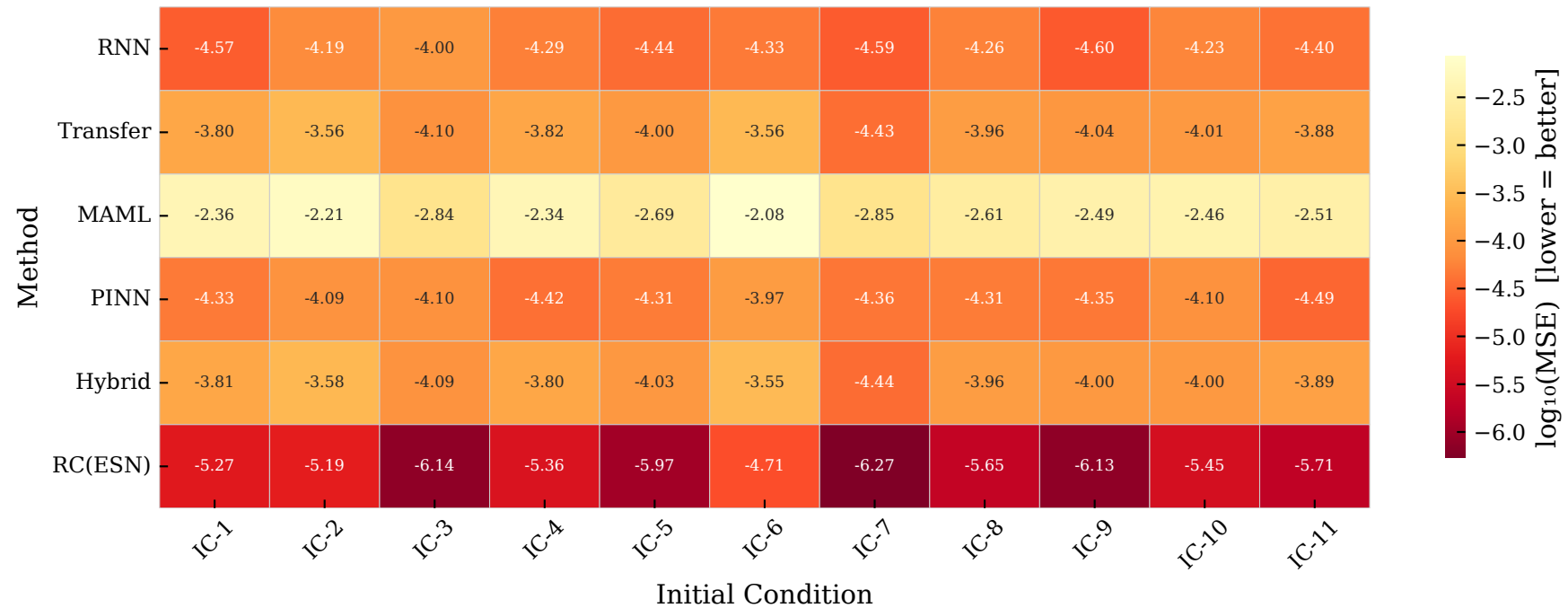
KS — \log_{10}(\text{MSE}) Heatmap: Method \times IC [lower = better]
