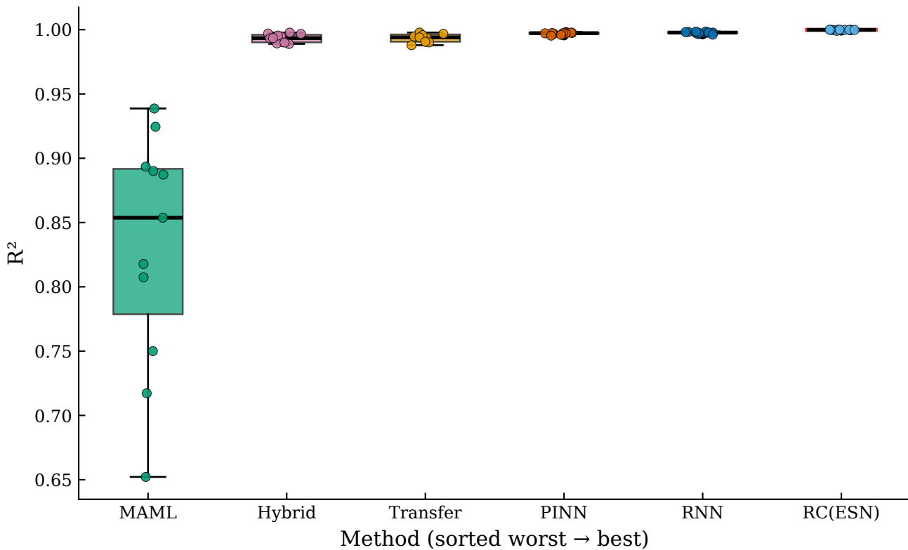
KS — R^2 Distribution (stable ICs)
