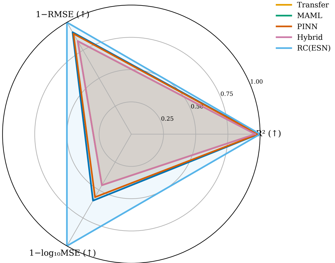
KS — Multi-Metric Radar (stable ICs)
