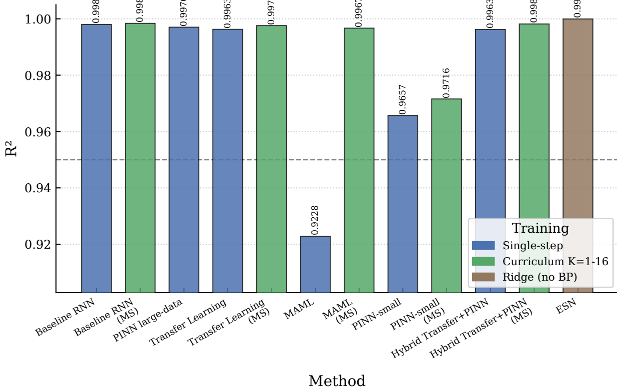
KS | R 2 Score: All Variants
