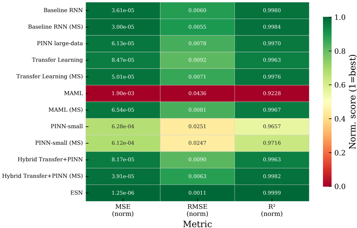
KS — Normalised Metric Heatmap (Green=best)
