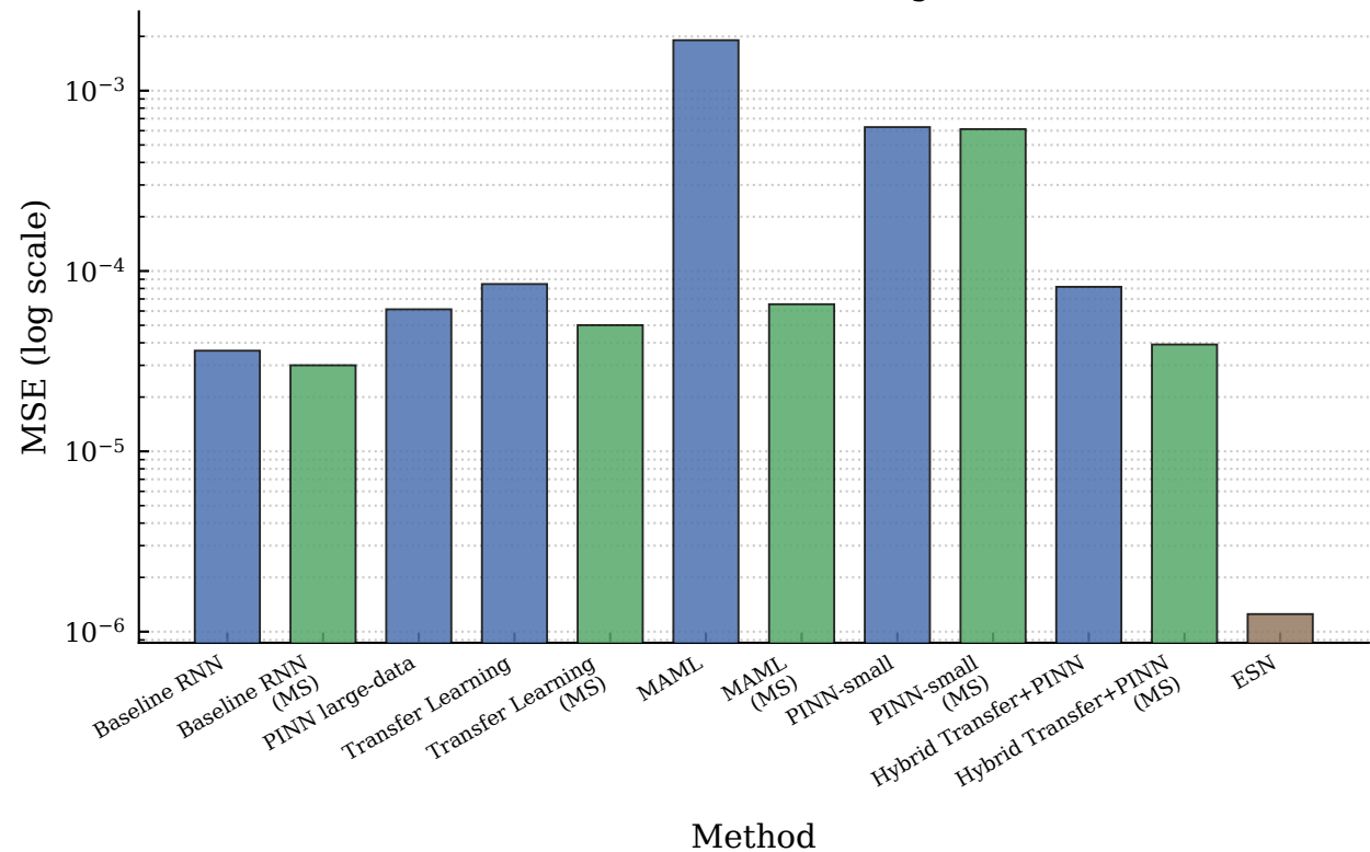
KS — MSE: All Variants (log scale)
