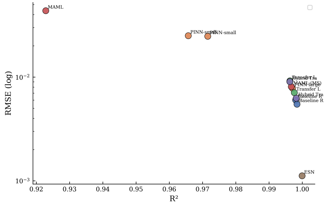
KS — RMSE vs R^2 with Pareto Frontier
