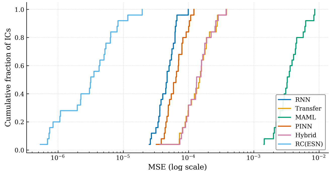
KS — Empirical CDF of MSE per Method
