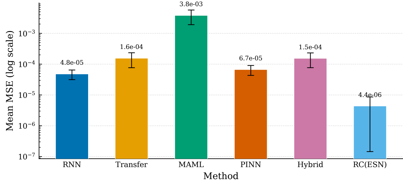
KS — Mean MSE Across 25 Random ICs
