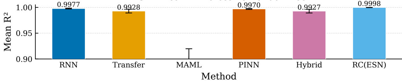
KS — Mean R^2 Across 25 Random ICs
