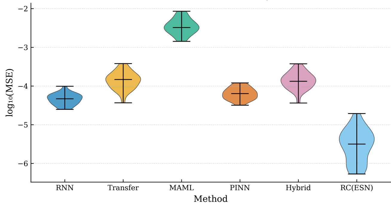
KS — MSE Distribution Shape ( \log_{10} scale)
