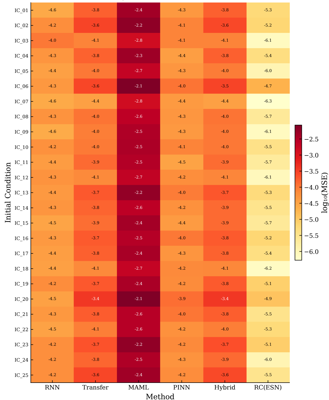
KS — \log_{10}(\text{MSE}) per IC and Method
