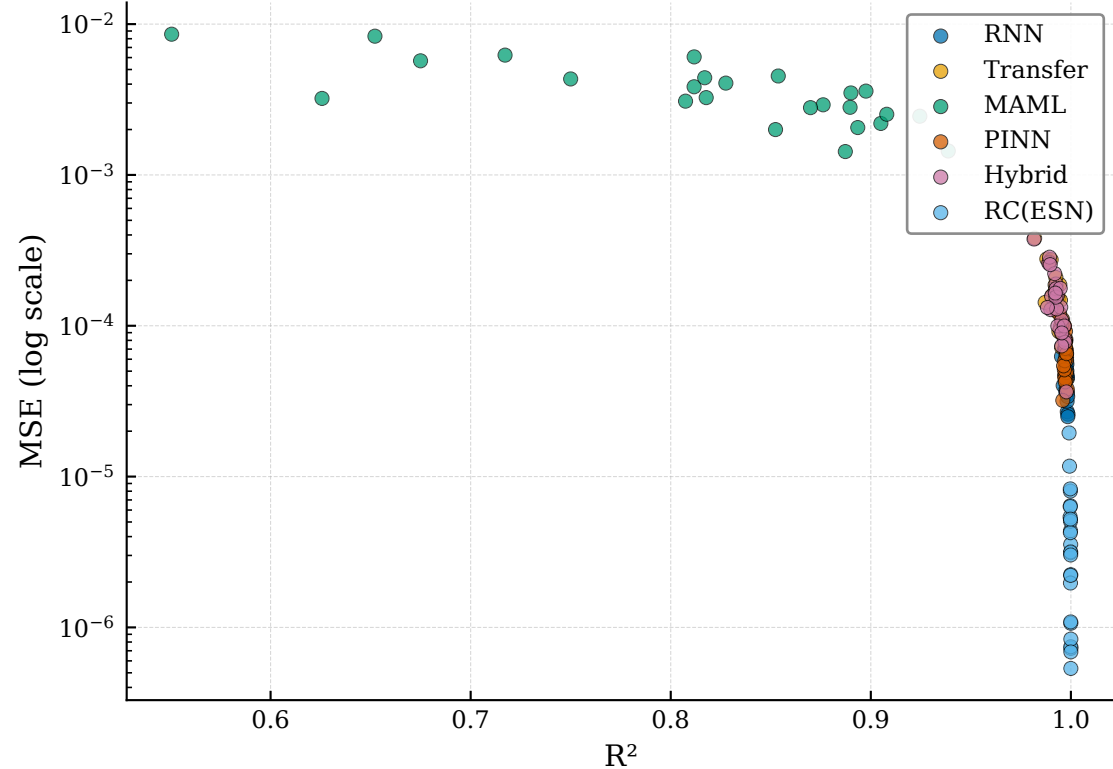
KS — MSE vs R^2 for All Methods and Random ICs
