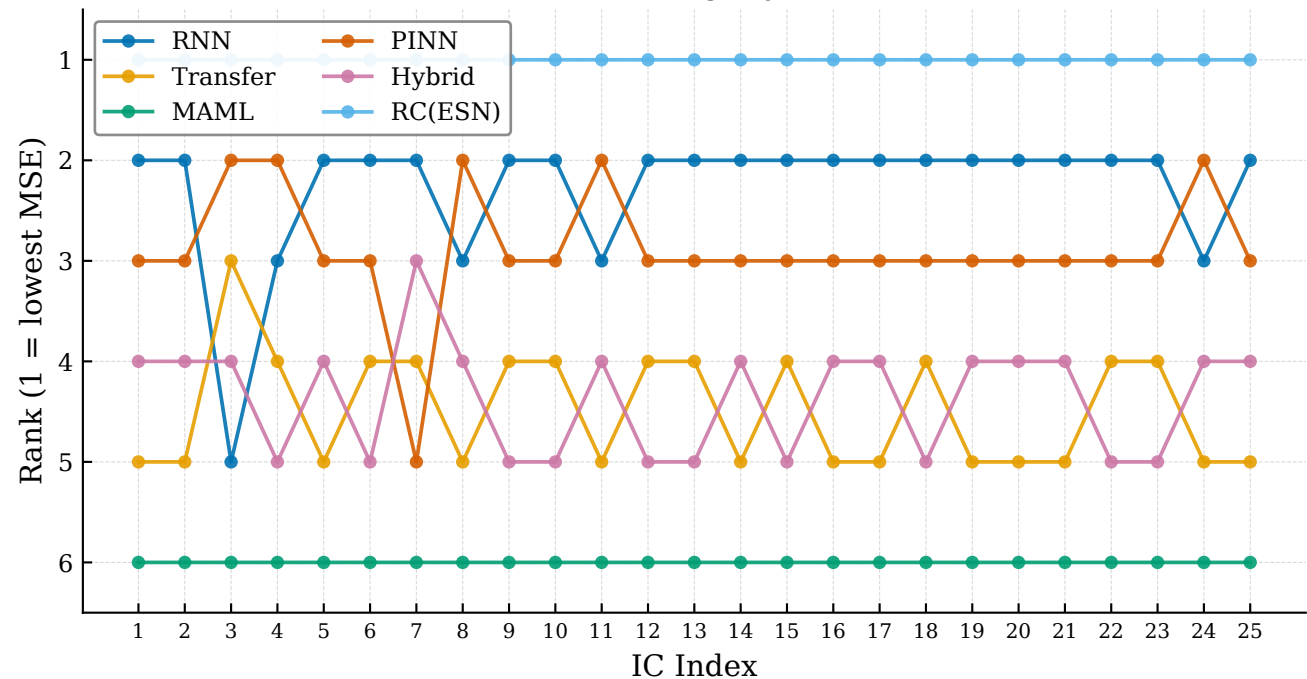
KS — Per-IC Method Rankings by MSE (Rank 1 = Best)
