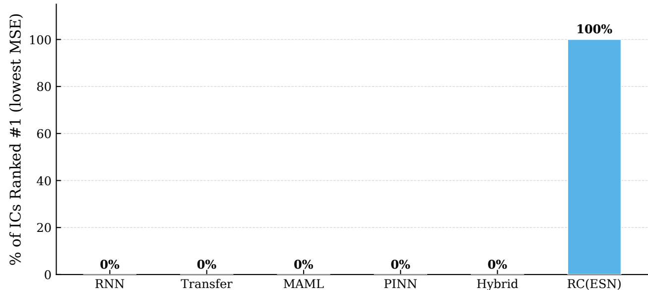
Lorenz — Fraction of Random ICs Where Method Achieves Lowest MSE
