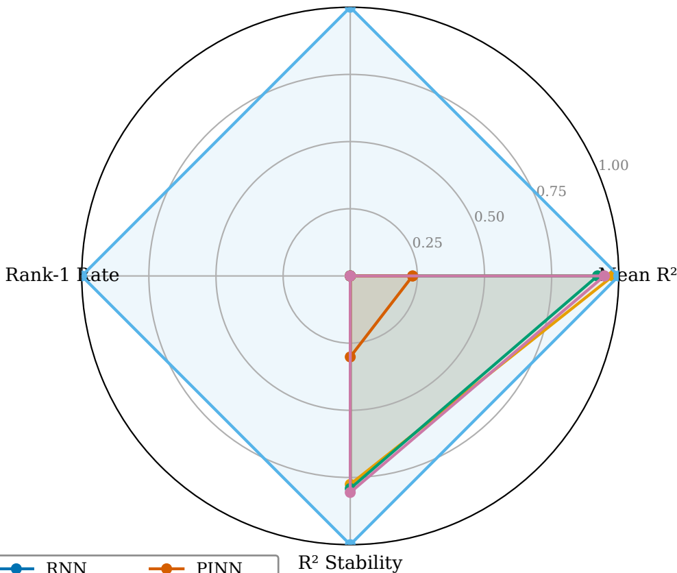
Lorenz — Multi-Metric Radar (Random ICs) 1/Mean MSE
