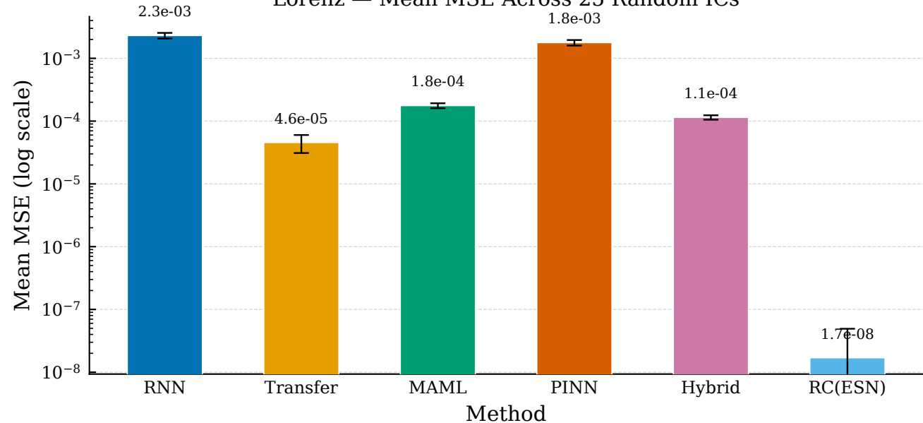
Lorenz — Mean MSE Across 25 Random ICs
