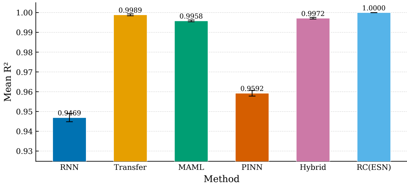
Lorenz — Mean R^2 Across 25 Random ICs
