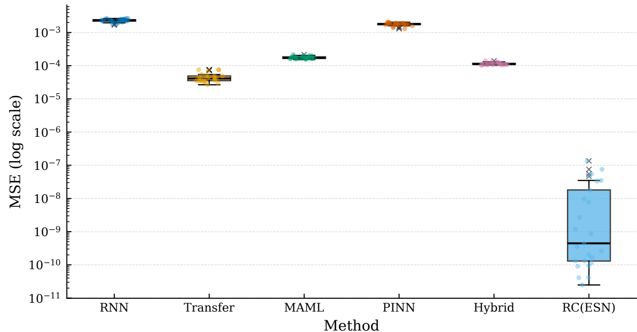
Lorenz — MSE Distribution Across 25 Random ICs
