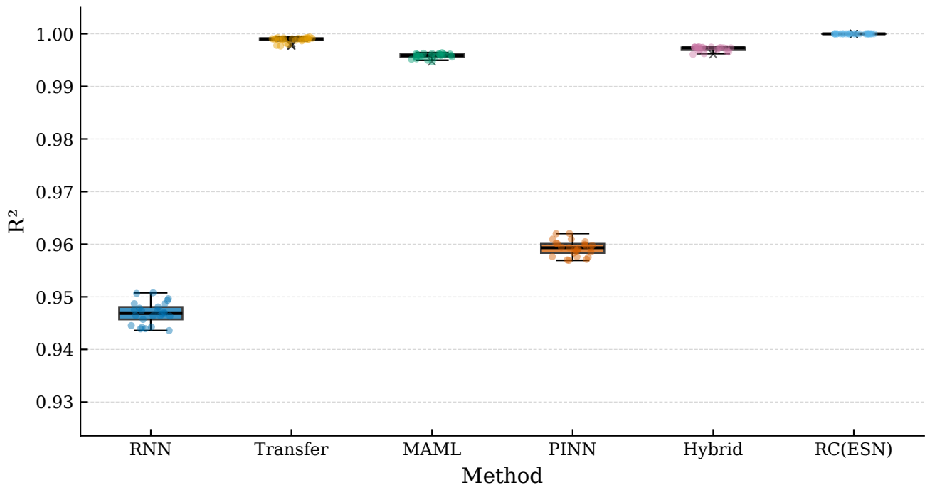
Lorenz — R^2 Distribution Across 25 Random ICs
